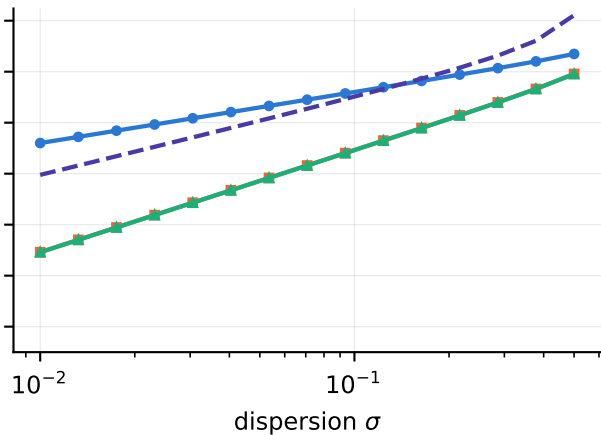
Cobb-Douglas frontier, symmetric inputs
