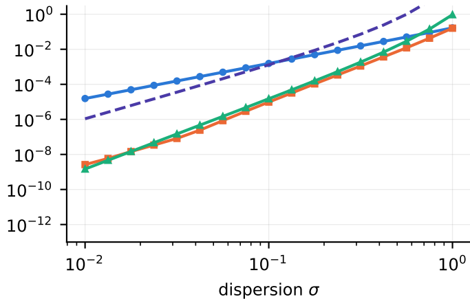
Cobb-Douglas frontier, log-normal inputs
