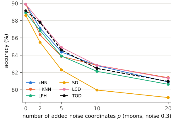
Figure 3: E2: accuracy against the number p of appended noise coordinates for five references and TOD (dashed); the best reference at each p is the highest line (HKNN, LCD).
