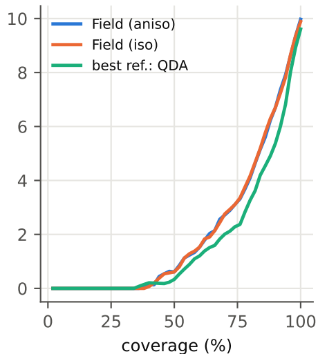
synth-classcov
