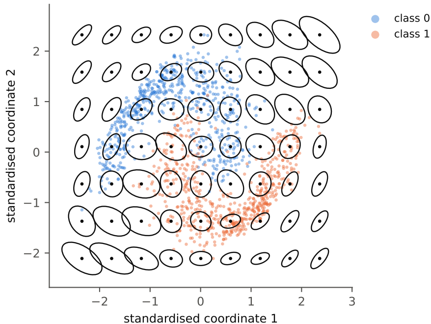
moons-aniso: neighbourhood ellipses ( K_m = 40 , \alpha = 0.2 ), 2-D projection
