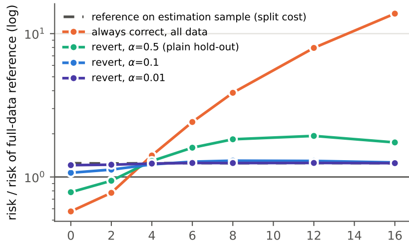
(a) with the guarantee of Theorem 4.2
