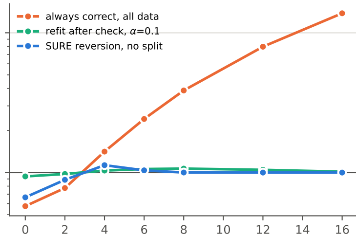
(b) without guarantee (empirical)
