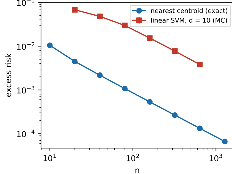
learning curves
