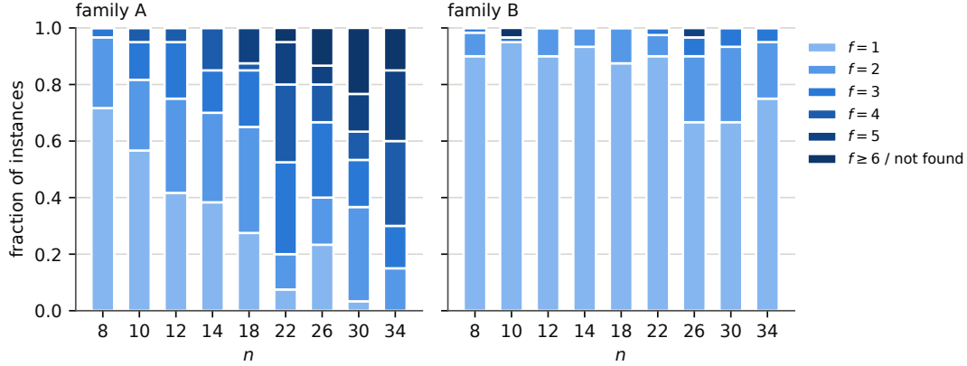
Figure 1: Distribution of the exact signed fragility number for ANY (rule C) as a function of n , families A and B, from E2 ( n \leq 14 ) and E4 ( n \geq 18 ; search capped at |R| \leq 6 , the top segment collects f \geq 6 and not found).
