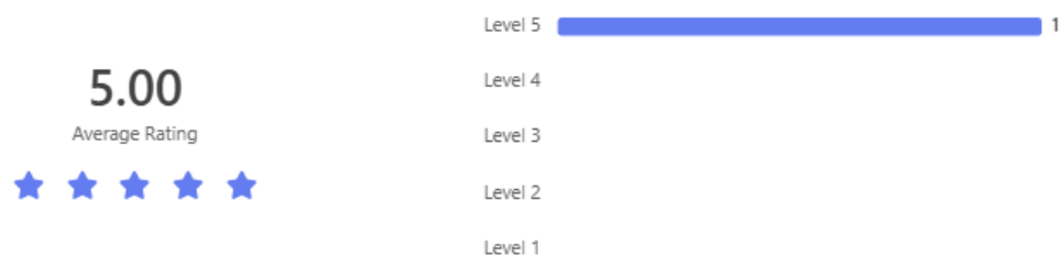
Figure 63: Task 6 Response
