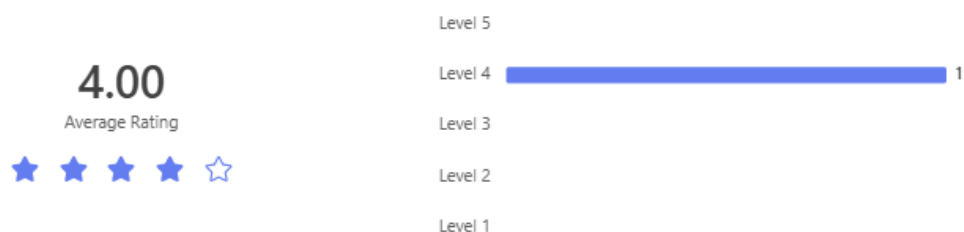
Figure 63: Q1 Response
