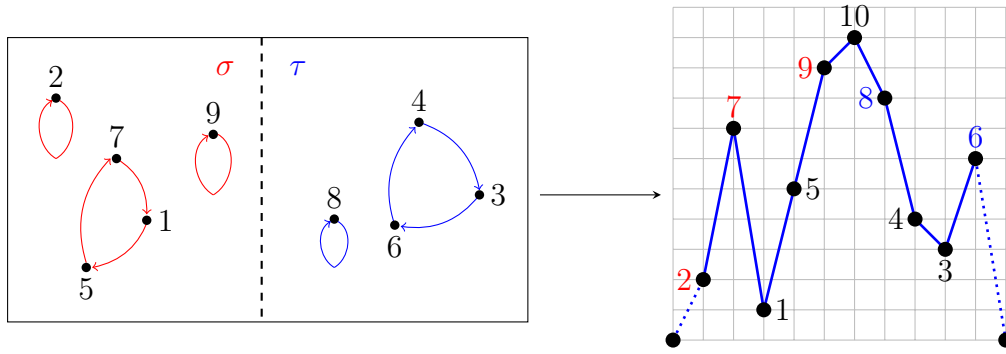
Figure 2.2: The mapping \rho : (\sigma, \tau) \mapsto \tilde{\pi} = 27159108436 .
