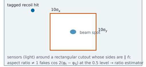
Schematic 3 — the coherent channel. Top: the far-forward measurement of the intact recoil, visible only when its transverse momentum carries it outside the beam envelope at the Roman Pots, and the vetoes that define exclusivity. Bottom left: the two physical azimuths relative to the alignment axis and the harmonic each mechanism modulates. Bottom right: the rectangular cutout, whose symmetry axes coincide with the spin axis.
