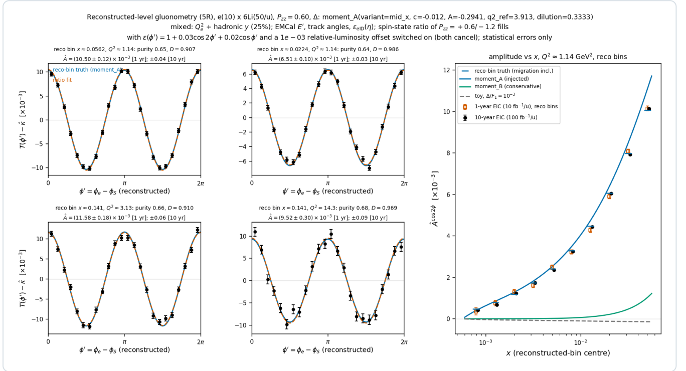
Money plot 5R — inclusive gluonometry at the reconstructed level ( e10 \times {}^6\text{Li}50 , P_{\text{ZZ}} = 0.6 , moment_A, mixed method with 25% hadronic y , ECal energy, track angles, \epsilon_{\text{eID}}(\eta) , spin-state ratio of the +0.6/-1.2 fills with the acceptance harmonic and luminosity offset on). Left: the acceptance-free modulation T(\phi') - \hat{k} per unit P_{\text{ZZ}} from the ratio, with the reco-bin truth (blue) and the fit (vermillion); annotations give purity, D and the 1-/10-year errors. Right: the amplitude in reconstructed x bins along the Q^2 = 1.14 \text{ GeV}^2 slice against the reco-bin truth (blue ticks) and the model curves.
