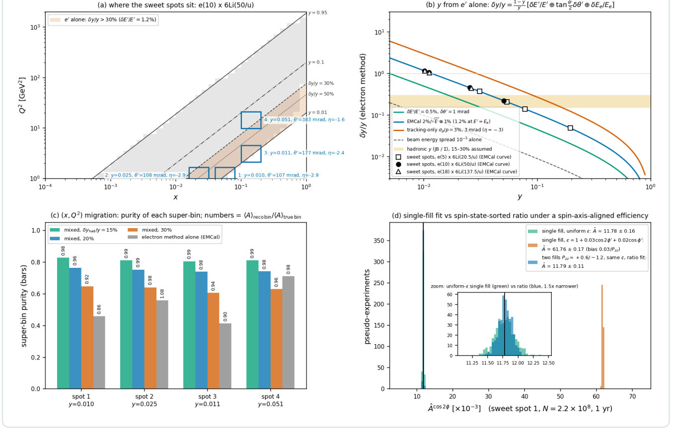
Figure 1 — the inclusive measurement quantified ( e(10) \times 6\text{Li}50 , reco_chain_figures.py ). (a) The analysis acceptance with iso- y lines and the four sweet-spot super-bins; the shaded band is where the electron alone gives \delta y/y > 30\% at a 1.2% energy resolution — spots 1–3 inside it, spot 4 just above. (b) The electron-method \delta y/y versus y for calorimeter, tracking and beam-energy-spread inputs, with the sweet spots of the three energies and the assumed 15–30% hadronic band. (c) Purity of each super-bin for three hadronic- y resolutions and for the electron method alone; the numbers give the amplitude averaged over the events landing in the reconstructed bin over that of the true bin. (d) Four hundred pseudo-experiments of the spot-1 super-bin at 1-year statistics: single-fill fit with a uniform efficiency (green), the same under \epsilon = 1 + 0.03 \cos 2\phi' + 0.02 \cos \phi' (vermillion, biased by 0.03/P_{zz} ) and the two-fill ratio fit under that efficiency (blue, unbiased and 1.5\times more precise; inset).
