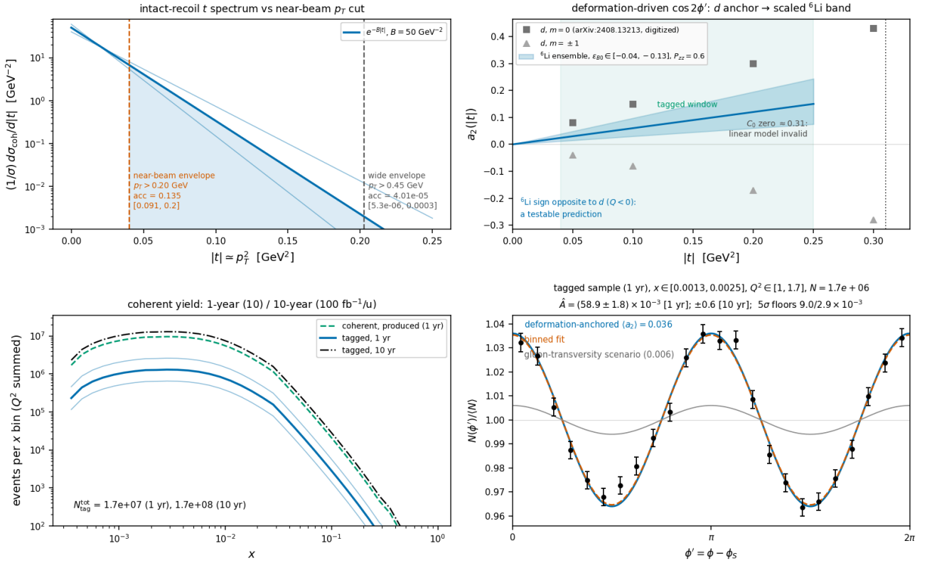
Figure 5 — the coherent channel e^6\text{Li} \rightarrow e'X^6\text{Li(g.s.)} at e(10) \times 6\text{Li}(99.5 \text{ GeV}/u) , P_{zz} = 0.60 , for a 0.20 GeV near-beam envelope. (a) Recoil t spectrum with the slope band and the 0.20 and 0.45 GeV cuts ( 13.5\% and 4 \times 10^{-5} ); the panel's optics labels are the proton optics the two cuts were first derived from, neither of which is an available ^6\text{Li} optics ( \$6.1 ). (b) Digitized deuteron a_2 per m state [10] against the scaled ^6\text{Li} ensemble band (sign flip predicted), with the tagged window and the form-factor-zero exclusion. (c) Tagged yield versus x for both programmes with the f_0 band. (d) \phi' pseudo-data (one-year statistics) at \langle a_2 \rangle = 0.036 with the flat gluon-transversity scenario (grey); extraction \hat{A} \pm 1.8 \times 10^{-3} (one year), \pm 0.6 \times 10^{-3} (ten years) per unit P_{zz} .
