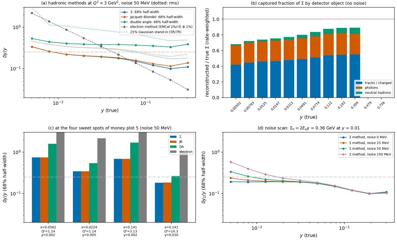
Figure 3 — hadronic-method resolution with a hadronic final state (e10 x ^6\text{Li} 50, PYTHIA 8 , 4 M e + p and e + n events, hfs_resolution.py ). (a) \delta y/y (68% half-width; dotted: rms) of the \Sigma , Jacquet-Blondel and double-angle methods at Q^2 < 3 \text{ GeV}^2 with the default response and 50 MeV noise, against the electron method and the 25% stand-in. (b) Captured fraction of \Sigma by detector object, no noise. (c) The four sweet spots. (d) The \Sigma -method resolution for 0, 25, 50 and 100 MeV of calorimeter noise.
