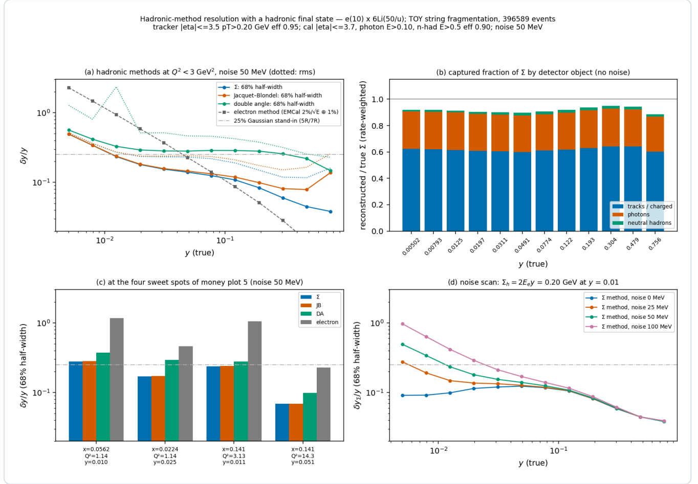
Figure 3 — hadronic-method resolution with a hadronic final state ( e10 \times {}^6\text{Li}50 , toy string fragmentation, hfs_resolution.py ; illustrative until the PYTHIA 8 sample is generated). (a) \delta y/y (68% half-width; dotted: rms) of the \Sigma , Jacquet–Blondel and double-angle methods at Q^2 < 3 \text{ GeV}^2 with the default response and 50 MeV noise, against the electron method and the 25% stand-in. (b) Captured fraction of \Sigma by detector object, no noise. (c) The four sweet spots of money plot 5. (d) The \Sigma -method resolution for calorimeter noise of 0, 25, 50 and 100 MeV: at y \approx 0.01 the noise floor, not the fragmentation, sets the resolution.
