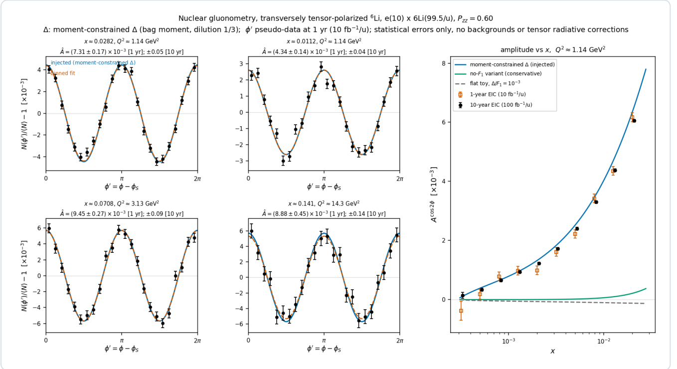
Figure 3 — projected extraction of \Delta \cos 2\phi pseudo-data (one EIC year, P_{zz} = 0.6 ) in the four highest-significance (x, Q^2) bins, with the injected moment-constrained \Delta model and the binned fit; right, the extracted amplitude versus x against alternative model readings. The precision distinguishes between the models rather than only from zero. The reconstructed-level version uses the spin-state ratio in reconstructed bins [5].
