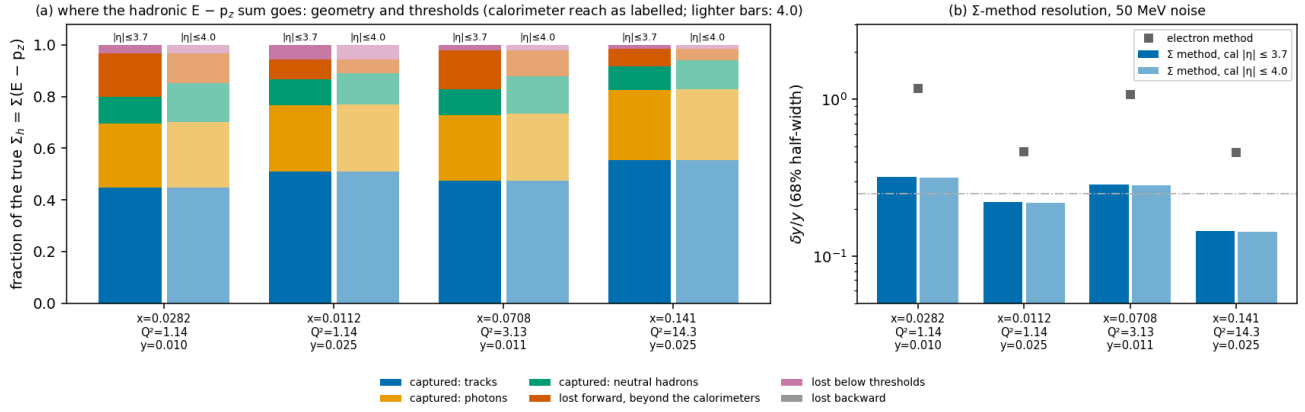
Figure 2 — where the hadronic E - p_z sum goes (e10 x ^6\text{Li} 99.5, PYTHIA 8, hfs_acceptance.py ). (a) The true \Sigma_h by fate — captured as tracks, photons and HCal objects; lost forward beyond the calorimeters, below threshold, or backward — for a calorimeter reach of |\eta| \leq 3.7 (full) and the ePIC nominal 4.0 (light). (b) The \Sigma -method \delta y/y through the full response for both reaches: the extra reach moves the bias, not the resolution.
