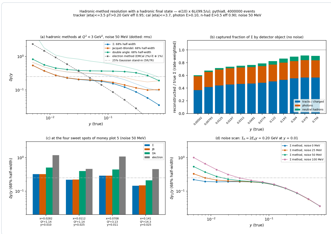
Figure 1 — hadronic-method resolution (e10 \times 6 Li99.5, PYTHIA 8, hfs_resolution.py ). (a) \delta y/y (68% half-width; dotted: rms) of the \Sigma , Jacquet-Blondel and double-angle methods at Q^2 < 3 GeV 2 with 50 MeV of noise, against the electron method and the 25% stand-in of the earlier chain. (b) Captured fraction of \Sigma by detector object, rate-weighted, no noise. (c) The four sweet spots. (d) The \Sigma -method resolution for 0, 25, 50 and 100 MeV of noise: the floor decides the y \approx 0.01 bins.
