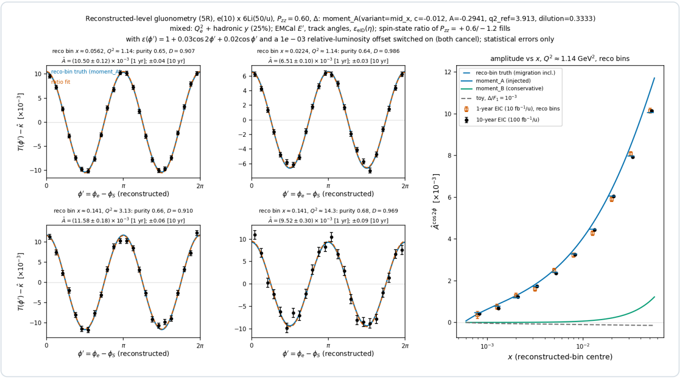
Money plot 5R — inclusive gluonometry at the reconstructed level ( e(10) \times {}^6\text{Li}50 , P_{zz} = 0.6 , moment_A, mixed method with 25% hadronic y , ECal energy, track angles, \epsilon_{\text{eID}}(\eta) , spin-state ratio of P_{zz} = +0.6/-1.2 fills with the acceptance harmonic and luminosity offset on). Left: the acceptance-free modulation T(\phi') - \hat{\kappa} (per unit P_{zz} ) from the ratio, with the reco-bin truth (blue) and the fit (vermillion); annotations give purity, D , and the 1-/10-year errors. Right: the amplitude in reconstructed x bins along the Q^2 = 1.14 \text{ GeV}^2 slice with the reco-bin truth (blue ticks) and the model curves.
