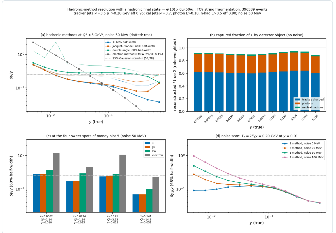
Figure 3 — hadronic-method resolution with a hadronic final state ( e(10) \times {}^6\text{Li}50 , toy string fragmentation, hfs_resolution.py ; illustrative until the PYTHIA 8 sample is generated). (a) \delta y/y (68% half-width; dotted: rms) of the \Sigma , Jacquet–Blondel and double-angle methods at Q^2 < 3 \text{ GeV}^2 with the default response and 50 MeV noise, against the electron method and the 25% stand-in. (b) Captured fraction of \Sigma by detector object, no noise. (c) The four sweet spots of money plot 5. (d) The \Sigma -method resolution for calorimeter noise of 0, 25, 50 and 100 MeV: at y \approx 0.01 the noise floor, not the fragmentation, sets the resolution.
