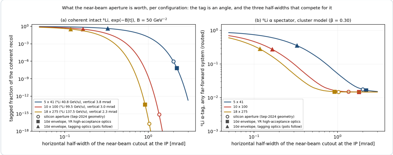
Figure 1 — the price of every aperture. Tagged fraction of the coherent intact {}^6\text{Li} (a, \exp(-B|t|) , B = 50 \text{ GeV}^{-2} ) and of the {}^6\text{Li} \alpha spectator routed through the far-forward systems (b, cluster model, \beta = 0.30 \text{ GeV} — the short-range parameter of the two-parameter cluster momentum density, whose 0.20–0.40 band is the model uncertainty) against the horizontal half-width of the near-beam cutout in angle, per configuration, with the vertical half-width fixed as in §1. Open circles: the silicon aperture of the September-2024 geometry; squares: the 10\sigma envelope of the Yellow Report high-acceptance optics; triangles: the envelope of the tagging optics. The curves are technology-independent and price any closer approach by any means; the markers are where the three constraints sit. nearbeam_aperture_scan.py .
