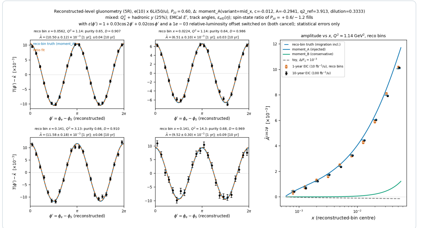
Money plot 5R — inclusive gluonometry at the reconstructed level ( e(10) \times {}^6\text{Li}(50, P_{zz} = 0.6, \text{moment\_A, mixed method with 25\% hadronic } y, \text{EMCal energy, track angles, } \epsilon_{\text{eID}}(\eta), \text{spin-state ratio of } P_{zz} = +0.6/-1.2 \text{ fills with the acceptance harmonic and luminosity offset on) ). Left: the acceptance-free modulation T(\phi') - \kappa' (per unit P_{zz} ) from the ratio, with the reco-bin truth (blue) and the fit (vermillion); annotations give purity, D , and the 1-/10-year errors. Right: the amplitude in reconstructed x bins along the Q^2 = 1.14 \text{ GeV}^2 slice with the reco-bin truth (blue ticks) and the model curves.
