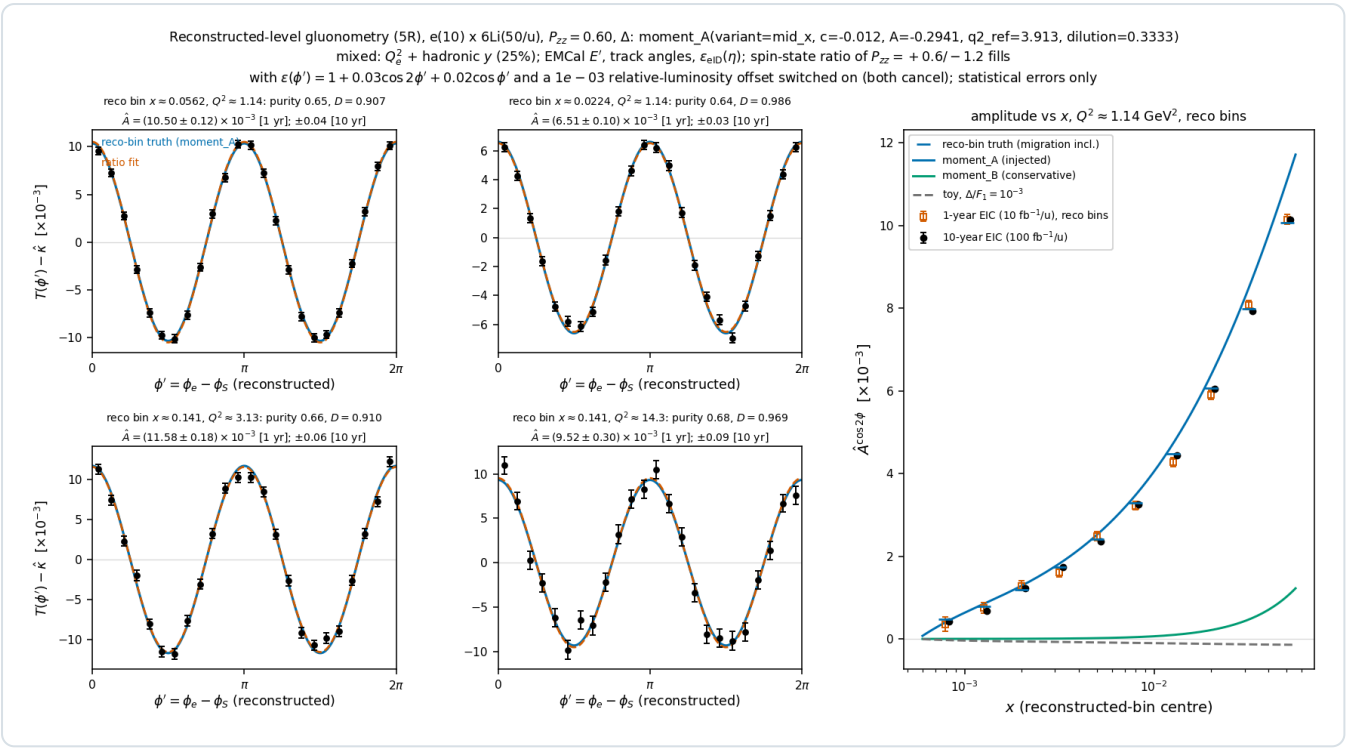
Money plot 5R — inclusive gluonometry at the reconstructed level ( e(10) \times {}^6\text{Li}(50/u) , P_{zz} = 0.6 , moment_A, mixed method with 25% hadronic y , EMCal energy, track angles, \epsilon_{\text{eID}}(\eta) , spin-state ratio of P_{zz} = +0.6/-1.2 fills with the acceptance harmonic and luminosity offset on). Left: the acceptance-free modulation \pi(\phi') - \hat{\kappa} (per unit P_{zz} ) from the ratio, with the reco-bin truth (blue) and the fit (vermillion); annotations give purity, D , and the 1-/10-year errors. Right: the amplitude in reconstructed x bins along the Q^2 = 1.14 \text{ GeV}^2 slice with the reco-bin truth (blue ticks) and the model curves.
