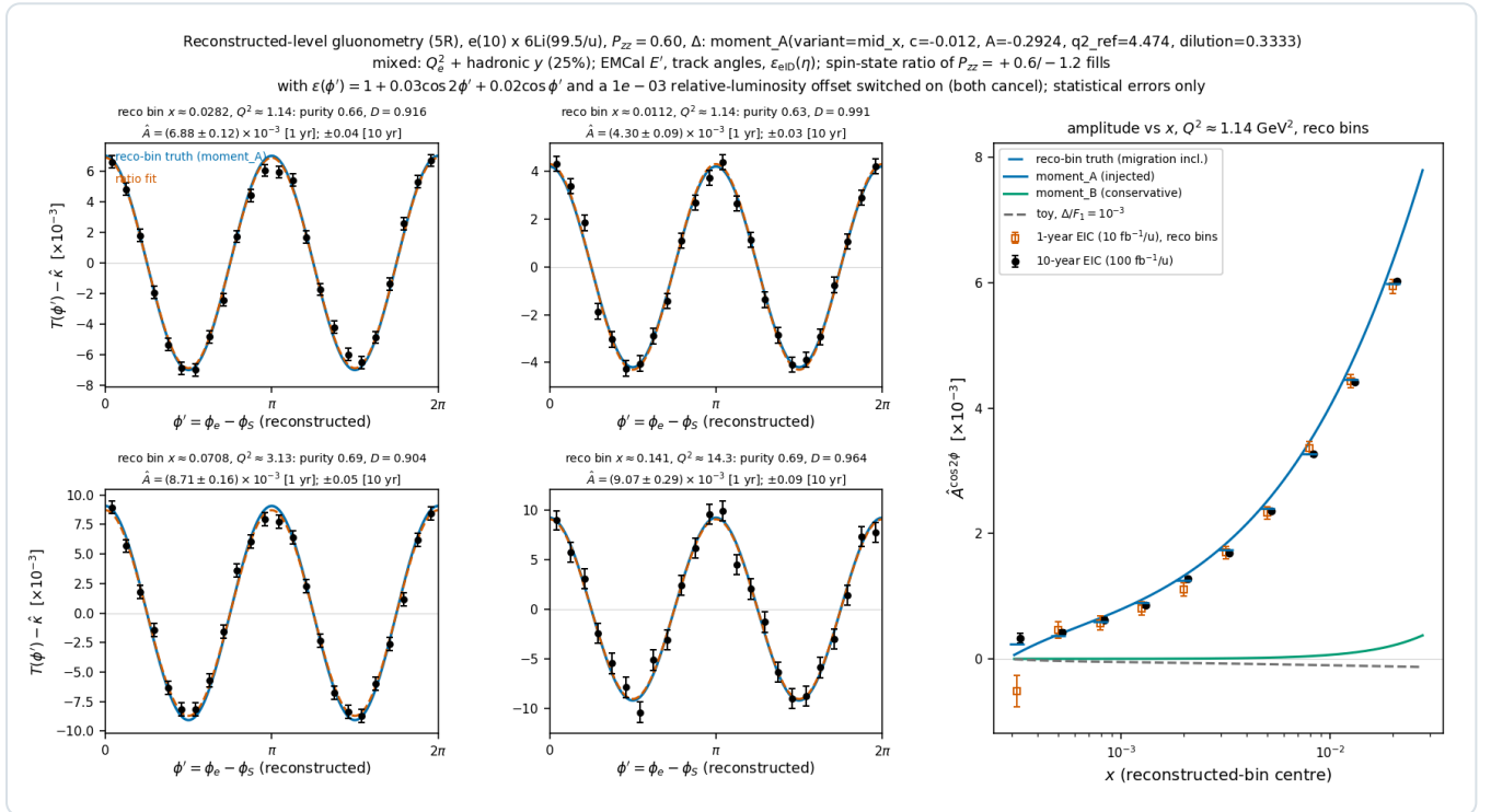
Money plot 5R — inclusive gluonometry at the reconstructed level ( e10 \times {}^6\text{Li}99.5 , P_{zz} = 0.6 , moment_A, mixed method with 25% hadronic y , EMCal energy, track angles, \epsilon_{\text{eID}}(\eta) , spin-state ratio of the +0.6/-1.2 fills with the acceptance harmonic and luminosity offset on). Left: the acceptance-free modulation T(\phi') - \hat{k} per unit P_{zz} from the ratio, with the reco-bin truth (blue) and the fit (vermillion); annotations give purity, D and the 1-/10-year errors. Right: the amplitude in reconstructed x bins along the Q^2 = 1.14 \text{ GeV}^2 slice against the reco-bin truth (blue ticks) and the model curves.
