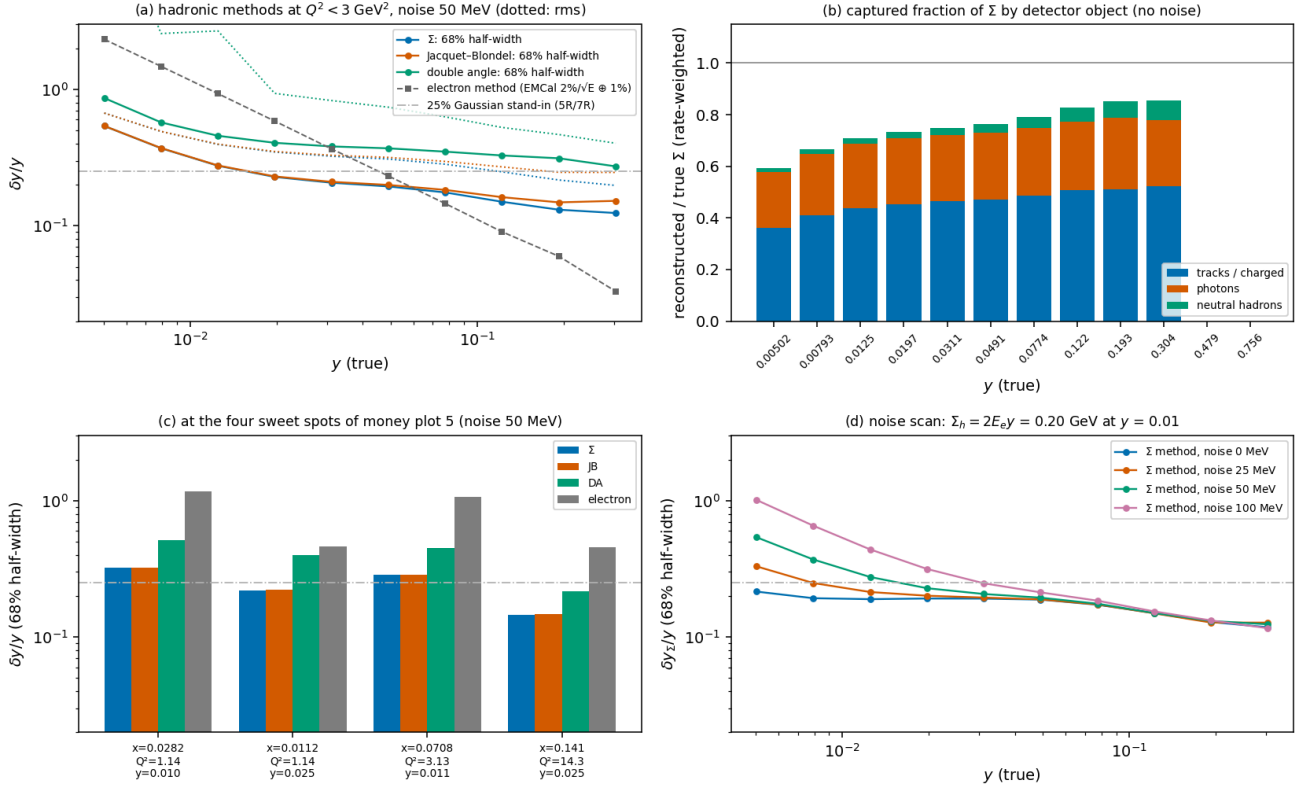
Figure 3 — hadronic-method resolution with a hadronic final state (e10 x 6Li99.5, PYTHIA 8, 4 M e + p and e + n events, hfs_resolution.py ). (a) \delta y/y (68% half-width; dotted: rms) of the \Sigma , Jacquet-Blondel and double-angle methods at Q^2 < 3 \text{ GeV}^2 with the default response and 50 MeV noise, against the electron method and the 25% stand-in. (b) Captured fraction of \Sigma by detector object, no noise. (c) The four sweet spots. (d) The \Sigma -method resolution for 0, 25, 50 and 100 MeV of calorimeter noise.
