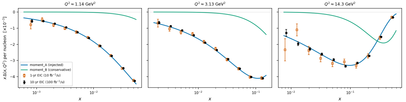
Money plot 7 — the extracted \Delta(x, Q^2) . The amplitudes of money plot 5 unfolded to the structure function (model bin-centering, \delta\Delta = \delta A \cdot |\partial\Delta/\partial A| ), as x\Delta per nucleon at the three sweet-spot Q^2 slices with independent 1-year (open) and 10-year (filled) pseudo-measurements against the moment_A and moment_B curves; the area under each curve is the ported bag moment ( \div 3 dilution). Best bins reach \delta\Delta \approx (0.7\text{--}1.4) \times 10^{-3} in year 1 on \Delta \approx -0.03\text{--}-0.09 .
