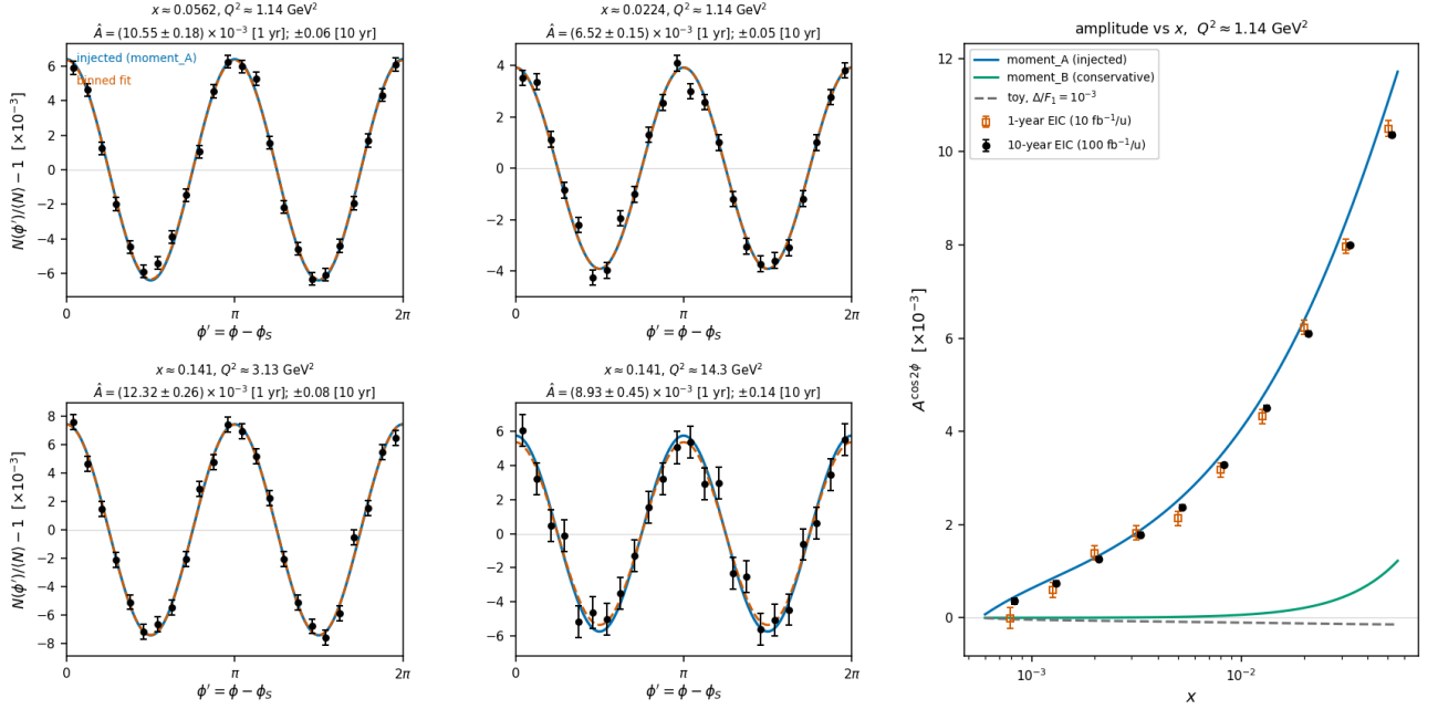
Money plot 5 — inclusive gluonometry ( e10 \times {}^6\text{Li}50 , P_{zz} = 0.60 , \Delta : moment_A, dilution 1/3). Left 2x2: \phi' pseudo-data with 1-year statistical error bars in the four sweet-spot super-bins ( Q^2 = 1.1 \rightarrow 14 \text{ GeV}^2 , x \approx 0.02\text{--}0.14 ); injected curve (blue), binned fit (vermillion); annotations give \delta A for both programs. Right: extracted amplitude vs x with 1-year (open) and 10-year (filled) error bars against the moment_A, moment_B and toy- 10^{-3} curves. Amplitudes are (0.7\text{--}1.2) \times 10^{-2} against \delta A = (1.5\text{--}4.5) \times 10^{-4} in year 1, i.e. every bin \geq 21\sigma , so the A-versus-B spread is resolved by the x dependence. Only the scattered electron is detected.
