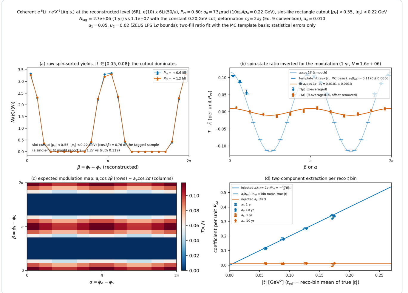
Money plot 6R — the coherent channel at the reconstructed level. (a) Raw spin-sorted yields versus the reconstructed recoil azimuth \beta for the lowest |t| bin: the slot-like cutout shape dominates both fills identically (vertical recoils, \beta \approx 0 and \pi , are the ones that clear the slot). (b) The modulation T(\beta) and T(\alpha) recovered from the spin-state ratio T(\alpha) with the a_t offset removed), the template-fit prediction per \beta bin (ticks) and the smooth a_t \cos 2\beta and a_e \cos 2\alpha curves. (c) The expected (noise-free) modulation map in (\alpha, \beta) : rows from the deformation term, columns from the gluon-transversity term. (d) Extracted a_t(t_{\text{ref}}) and a_e per reco |t| bin (1 yr open, 10 yr filled) against the injected curves.
