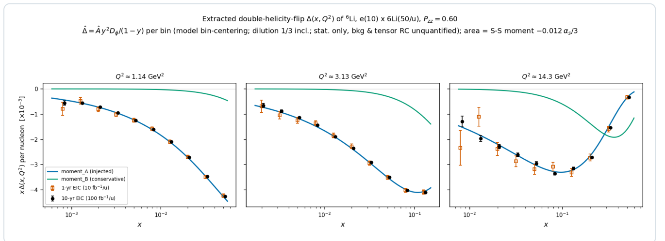
Money plot 7 — the extracted \Delta(x, Q^2) itself. The \cos 2\phi amplitudes of money plot 5 unfolded to the structure function, \hat{\Delta} = \hat{A} y^2 D_\phi / (1-y) per bin (model bin-centering; \delta \Delta = \delta A \cdot |\partial \Delta / \partial A| ), shown as x \Delta(x, Q^2) per nucleon at the three sweet-spot Q^2 slices with independent 1-year (open) and 10-year (filled) pseudo-measurements against the moment_A (blue) and moment_B (green) curves — the area under each curve is the Sather–Schmidt moment ( \pm 3 dilution). Best bins reach \delta \Delta \approx (0.7\text{--}1.4) \times 10^{-3} in year 1 on \Delta \approx -0.03\text{--}-0.09 ; the A -vs- B ansatz spread is resolved bin by bin.
