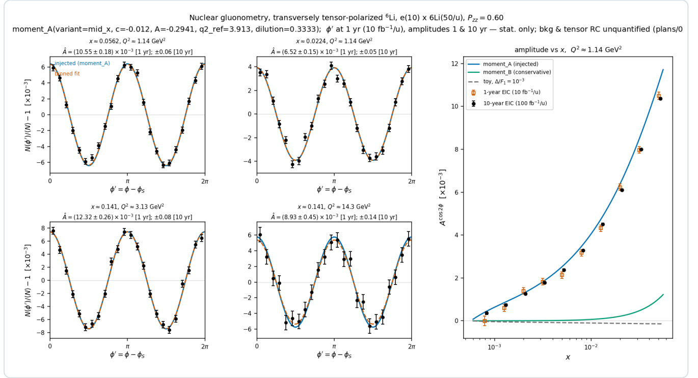
Money plot 5 — inclusive gluonometry ( e10 \times {}^6\text{Li}50 , P_{zz} = 0.60 , \Delta model: moment_A , dilution 1/3 ). Left 2 \times 2 : \phi' -modulation pseudo-data with statistical error bars at the 1-year program (10 fb ^{-1}/u ) in the four sweet-spot super-bins ( Q^2 = 1.1 \rightarrow 14 \text{ GeV}^2 , x \approx 0.02\text{--}0.14 ); injected curve (blue), binned fit (vermillion); per-panel annotations give \delta A for both programs. Right: extracted amplitude vs x with 1-year (open) and 10-year (filled) error bars against the moment_A (blue), moment_B (green), and toy - 10^{-3} (gray) curves. Amplitudes are (0.7\text{--}1.2) \times 10^{-2} at the sweet spots against \delta A = (1.5\text{--}4.5) \times 10^{-4} in year 1 — every bin \geq 21\sigma , so the A -vs- B ansatz spread is resolved by the x -shape. Detection needs only the scattered electron.
