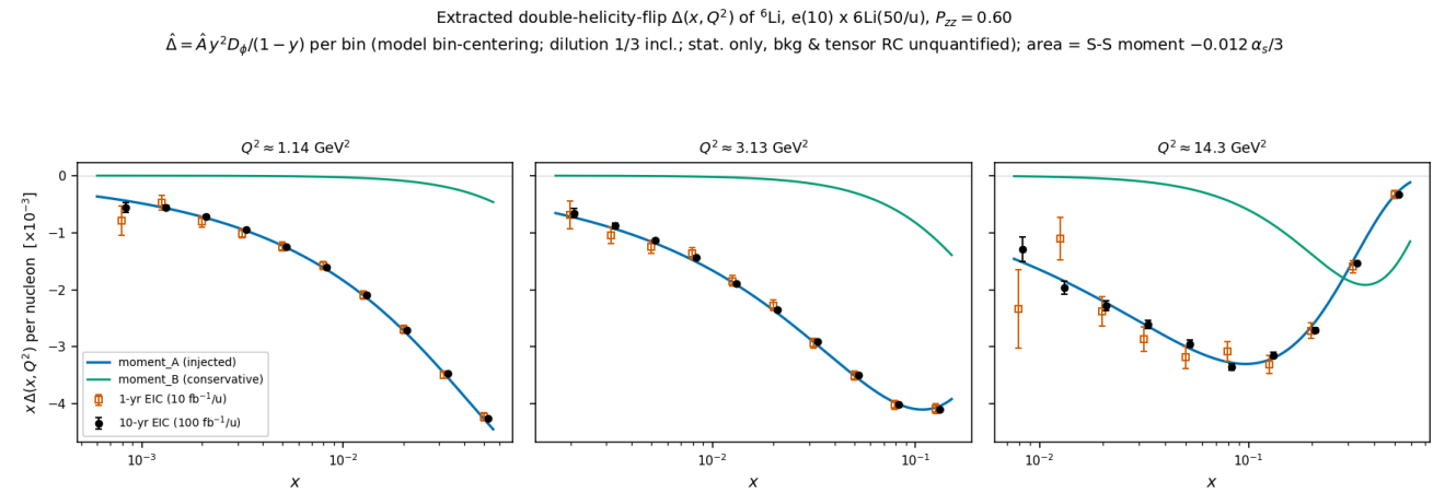
Money plot 7 — the extracted \Delta(x, Q^2) itself. The \cos 2\phi amplitudes of money plot 5 unfolded to the structure function, \hat{\Delta} = \hat{A} y^2 D_{\phi}/(1-y) per bin (model bin-centering; \delta \Delta = \delta A |\partial \Delta / \partial A| ), shown as x \Delta(x, Q^2) per nucleon at the three sweet-spot Q^2 slices with independent 1-year (open) and 10-year (filled) pseudo-measurements against the moment_A (blue) and moment_B (green) curves — the area under each curve is the Sather–Schmidt moment ( \div 3 dilution). Best bins reach \delta \Delta \approx (0.7 – 1.4) \times 10^{-3} in year 1 on \Delta \approx -0.03 ... -0.09 ; the A-vs-B ansatz spread is resolved bin by bin.
