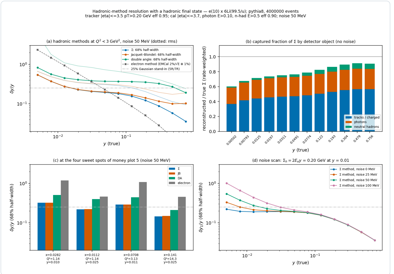
Figure 3 — hadronic-method resolution ( e(10) \times {}^6\text{Li}99.5 , PYTHIA 8, hfs_resolution.py ). (a) \delta y/y (68% half-width; dotted: rms) of the \Sigma , Jacquet-Blondel and double-angle methods at Q^2 < 3 \text{ GeV}^2 with 50 MeV of noise, against the electron method and the 25% stand-in of the earlier chain. (b) Captured fraction of \Sigma by detector object, rate-weighted, no noise. (c) The four sweet spots. (d) The \Sigma -method resolution for 0, 25, 50 and 100 MeV of noise: the floor decides the y \approx 0.01 bins.
