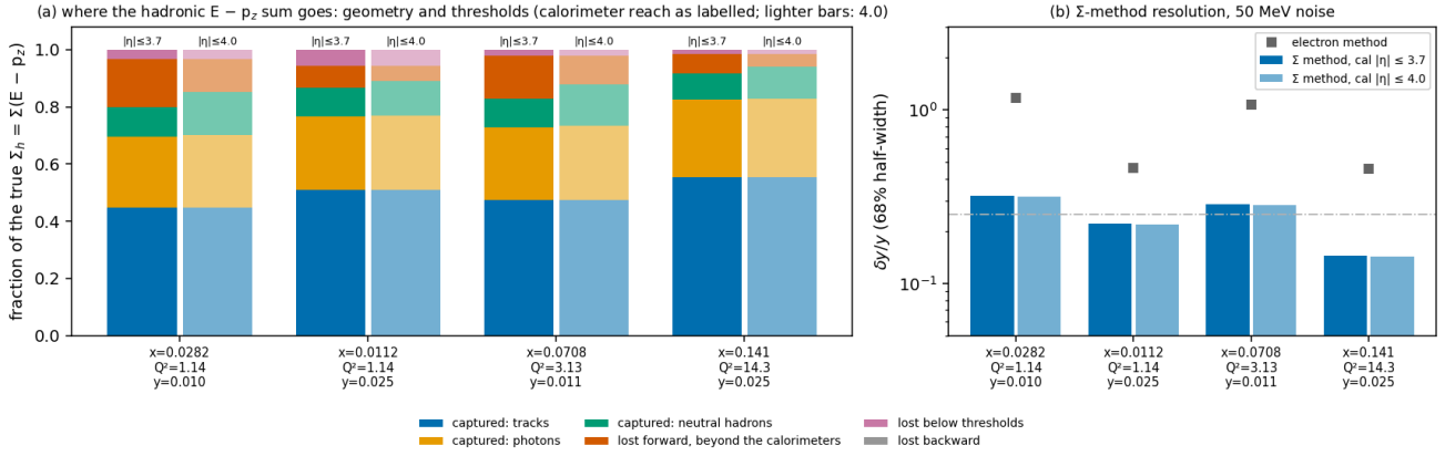
Figure 4 — where the hadronic E - p_z sum goes (e10 x ^6\text{Li} 99.5, PYTHIA 8, hfs_acceptance.py ). (a) The true \Sigma_h by fate — captured as tracks, photons and HCal objects; lost forward beyond the calorimeters, below threshold, or backward — for a calorimeter reach of |\eta| \leq 3.7 (full) and the ePIC nominal 4.0 (light). (b) The \Sigma -method \delta y/y through the full response for both reaches: the extra reach moves the bias, not the resolution.
