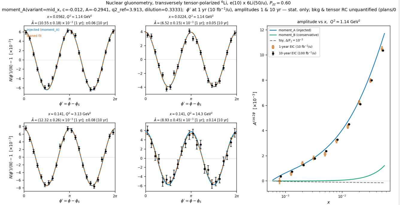
Money plot 5 — inclusive gluonometry ( e(10) \times {}^6\text{Li}50 , P_{zz} = 0.60 , \Delta model: moment_A, dilution 1/3). Left 2x2: \phi' -modulation pseudo-data with statistical error bars at the 1-year program (10 fb ^{-1} /u) in the four sweet-spot super-bins ( Q^2 = 1.1 \rightarrow 14 \text{ GeV}^2 , x \approx 0.02\text{--}0.14 ); injected curve (blue), binned fit (vermillion); per-panel annotations give \delta A for both programs. Right: extracted amplitude vs x with 1-year (open) and 10-year (filled) error bars against the moment_A (blue), moment_B (green), and toy- 10^{-3} (gray) curves. Amplitudes are (0.7\text{--}1.2) \times 10^{-2} at the sweet spots against \delta A = (1.5\text{--}4.5) \times 10^{-4} in year 1 — every bin \geq 21\sigma , so the A-vs-B ansatz spread is resolved by the x-shape. Detection needs only the scattered electron.
