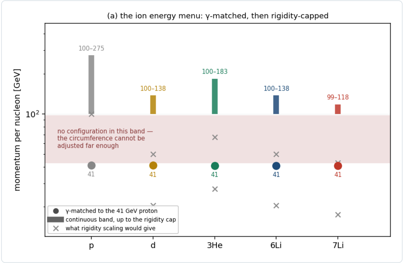
Figure 1 — the ion energy menu. Each species has an isolated \gamma -matched point at \approx 41 GeV/u and a continuous band from \approx 99 GeV/u to its own rigidity cap, with nothing between. Crosses mark what rigidity scaling would have given, which this programme used until 2026-08-27. eic_beam_figures.py .
