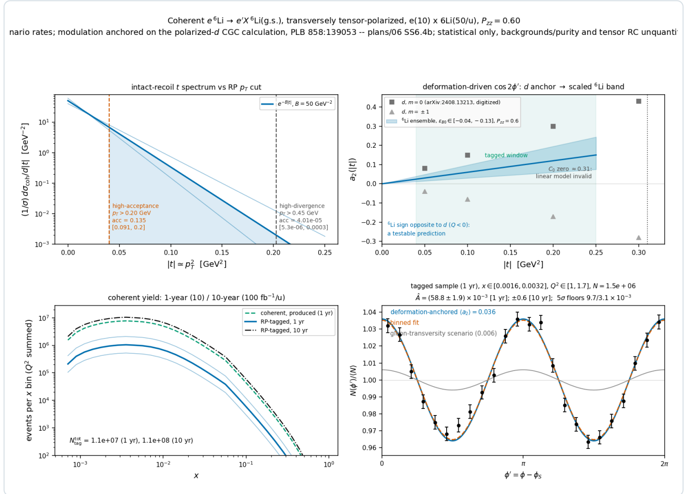
Money plot 6 — coherent channel, e^6\text{Li} \rightarrow e'X^6\text{Li}(\text{g.s.}) (same beam, P_{zz} = 0.60 ). Top left: recoil t -spectrum vs both optics' p_T cuts with the slope band. Top right: digitized deuteron a_2 per m -state [13] vs the scaled {}^6\text{Li} ensemble band (sign flip predicted); tagged window and form-factor-zero exclusion marked. Bottom left: tagged yield vs x for both programs with the f_0 band ( N_{\text{tag}} \approx 1.1 \times 10^7 / 1.1 \times 10^8 ). Bottom right: \phi' pseudo-data (1-year statistics) at the anchored \langle a_2 \rangle = 0.036 with the flat gluon-transversity scenario (gray); extraction \hat{A} \pm 1.9 \times 10^{-3} (1 yr), \pm 0.6 \times 10^{-3} (10 yr).
