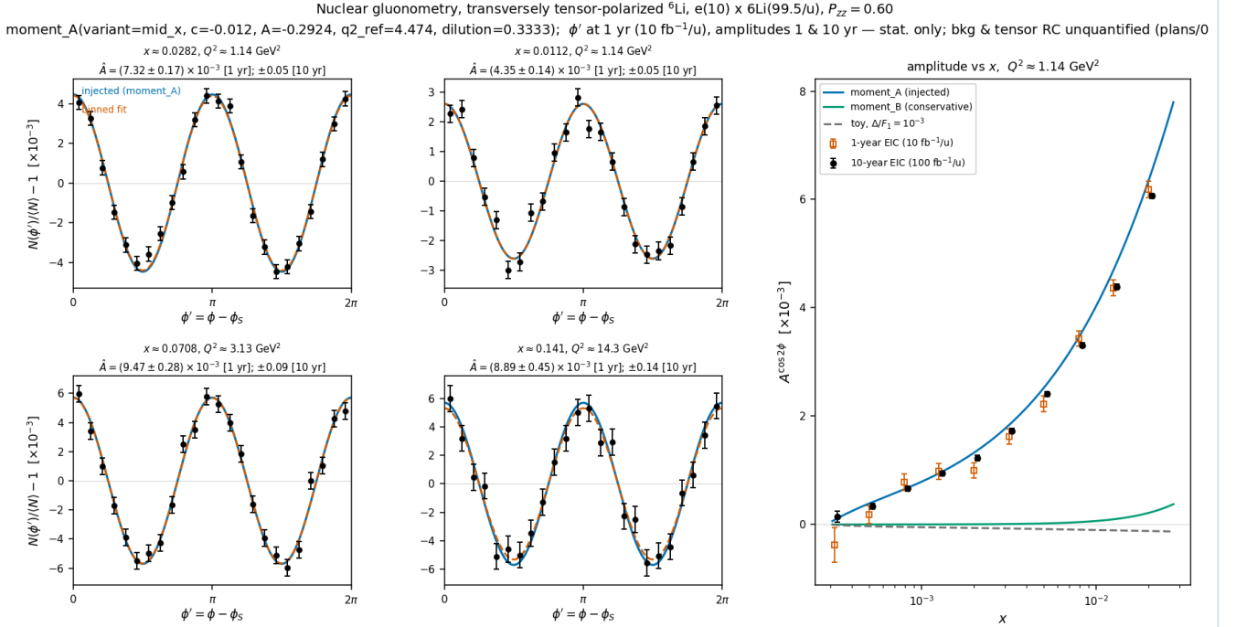
Money plot 5 — inclusive gluonometry ( e(10) \times {}^6\text{Li}50 , P_{zz} = 0.60 , \Delta : moment_A, dilution 1/3). Left 2x2: \phi' pseudo-data with 1-year statistical error bars in the four sweet-spot super-bins ( Q^2 = 1.1 \rightarrow 14 \text{ GeV}^2 , x \approx 0.02-0.14 ); injected curve (blue), binned fit (vermillion); annotations give \delta A for both programs. Right: extracted amplitude vs x with 1-year (open) and 10-year (filled) error bars against the moment_A, moment_B and toy- 10^{-3} curves. Amplitudes are (0.7-1.2) \times 10^{-2} against \delta A = (1.5-4.5) \times 10^{-4} in year 1, i.e. every bin \geq 21\sigma , so the A-versus-B spread is resolved by the x dependence. Only the scattered electron is detected.
