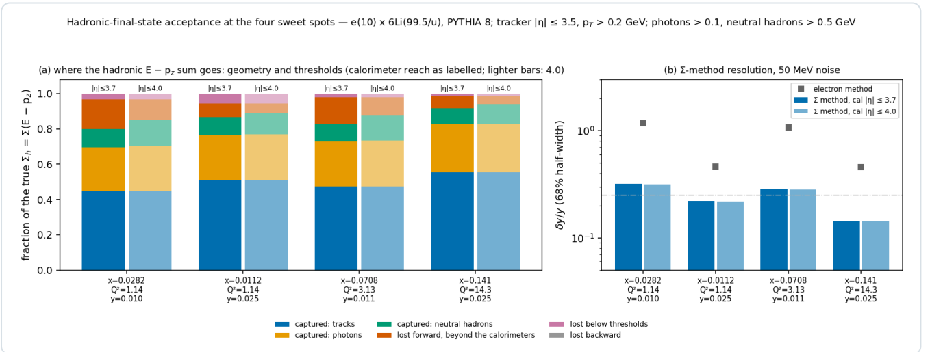
Figure 2 — where the hadronic E - p_z sum goes ( e(10) \times {}^6\text{Li}99.5 , PYTHIA 8, hfs_acceptance.py ). (a) The true \Sigma_h by fate — captured as tracks, photons and HCal objects; lost forward beyond the calorimeters, below threshold, or backward — for a calorimeter reach of |\eta| \leq 3.7 (full) and the ePIC nominal 4.0 (light). (b) The \Sigma -method \delta y/y through the full response for both reaches: the extra reach moves the bias, not the resolution.
