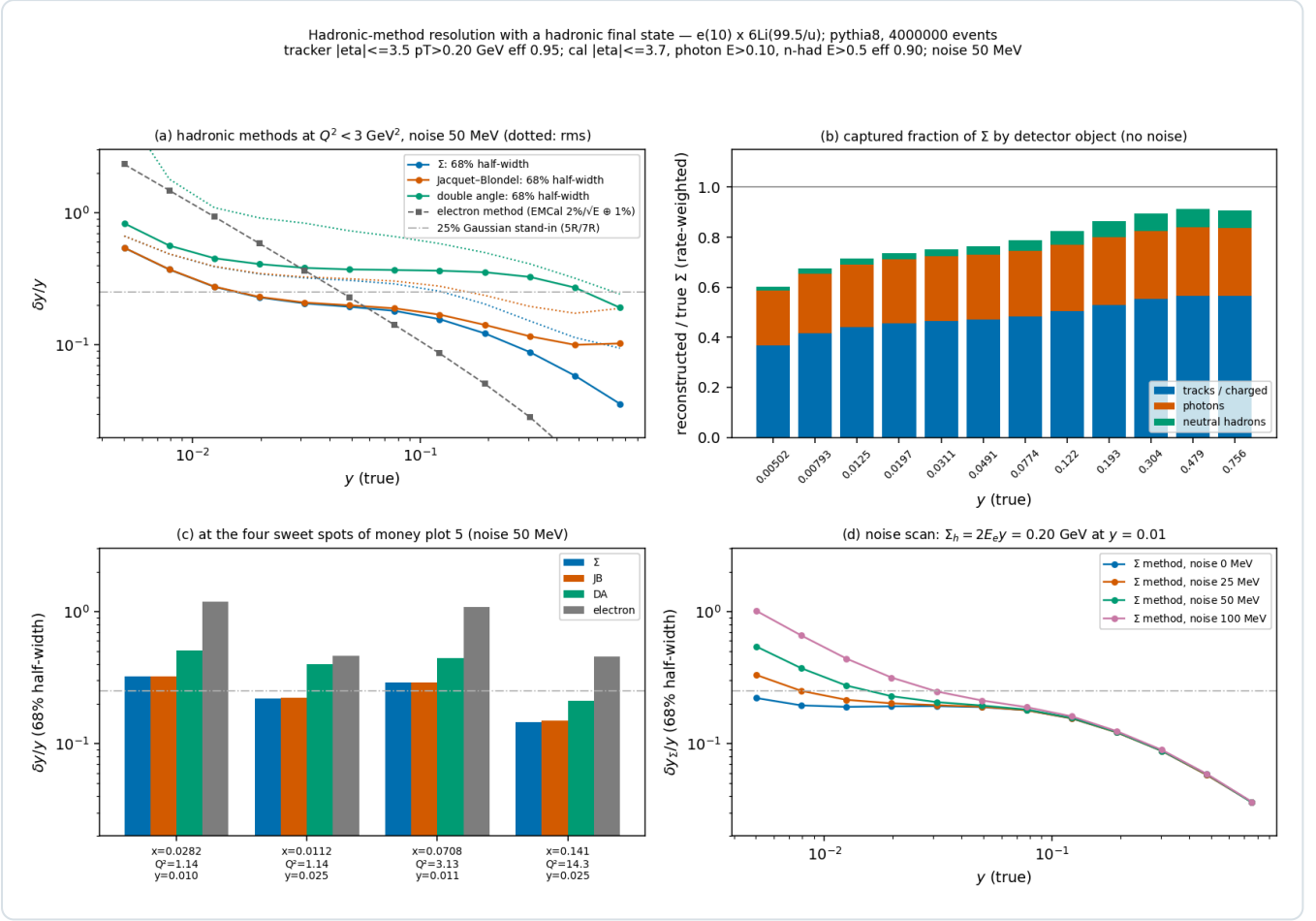
Figure 1 — hadronic-method resolution ( e(10) \times {}^6\text{Li}99.5 , PYTHIA 8, hfs_resolution.py ). (a) \delta y/y (68% half-width; dotted: rms) of the \Sigma , Jacquet-Blondel and double-angle methods at Q^2 < 3 \text{ GeV}^2 with 50 MeV of noise, against the electron method and the 25% stand-in of the earlier chain. (b) Captured fraction of \Sigma by detector object, rate-weighted, no noise. (c) The four sweet spots. (d) The \Sigma -method resolution for 0, 25, 50 and 100 MeV of noise: the floor decides the y \approx 0.01 bins.
