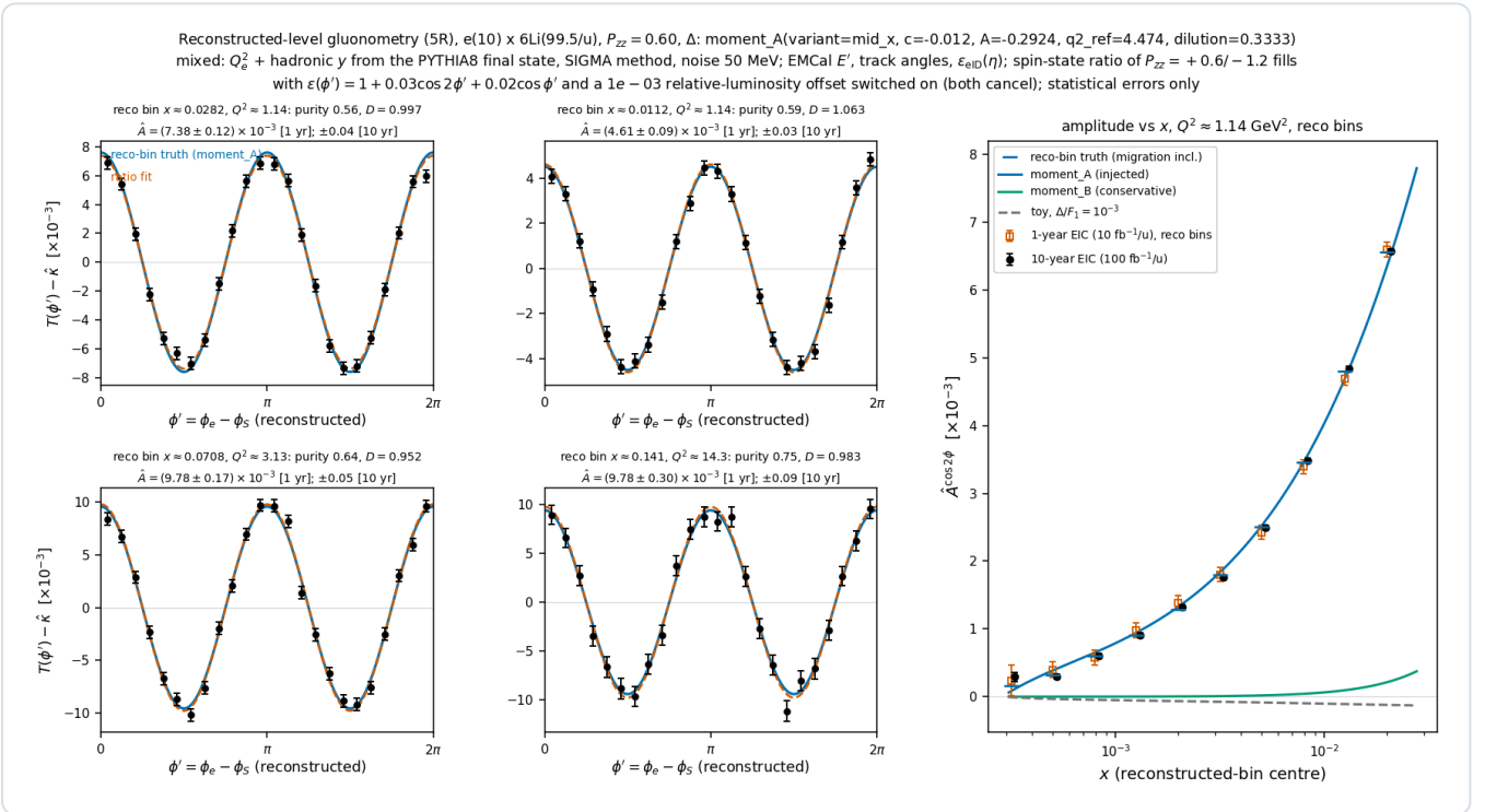
Money plot 5R — inclusive gluonometry at the reconstructed level (e10 × 6 Li99.5, P zz = 0.6, model A, PYTHIA 8 final state with the Σ method and the calibrated hadronic scale, EMCal energy, track angles, ε elD (η), spin-state ratio of the +0.6 / −1.2 states with the acceptance harmonic and luminosity offset on). Left: the acceptance-free modulation T(φ') − k̂ per unit P zz with the reconstructed-bin truth (blue) and the fit (vermillion). Right: the amplitude in reconstructed x bins along the Q 2 = 1.14 GeV 2 slice against the reconstructed-bin truth (blue ticks) and the model curves.
