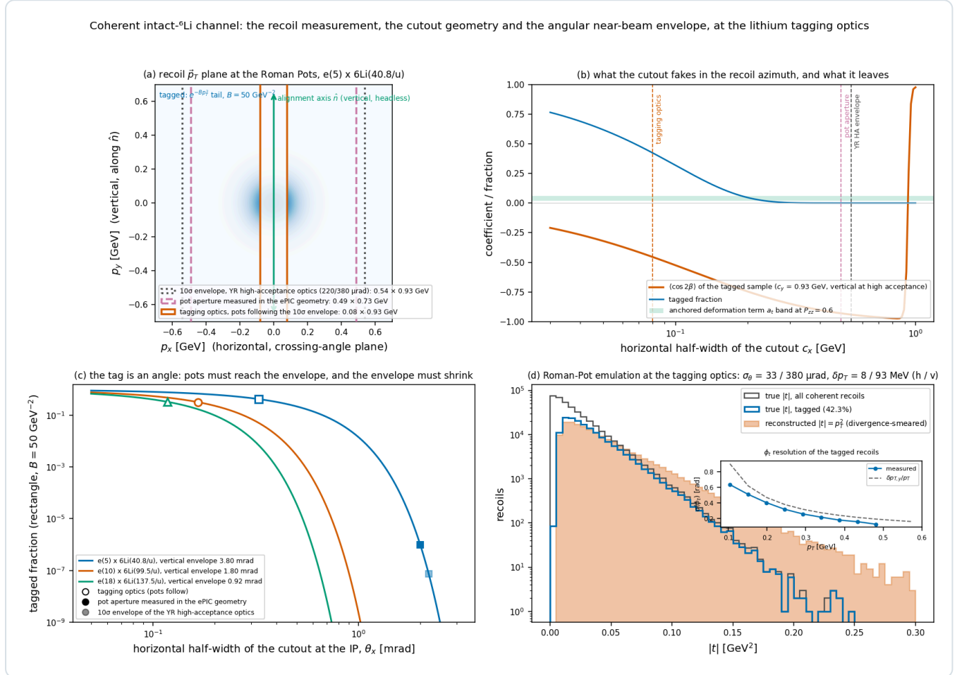
Figure 3 — the coherent measurement quantified (5 × 40.8, reco_chain_figures.py ). (a) The recoil p_T plane with the exponential coherent spectrum and the three cutouts: the Yellow Report high-acceptance 10 \sigma envelope, the pot aperture measured in the ePIC geometry, and the tagging optics with pots following the envelope. (b) \cos 2\beta of the tagged sample about the vertical spin axis and the tagged fraction versus the horizontal half-width of the cutout, against the anchored deformation band. (c) Tagged fraction versus the horizontal half-angle at the interaction point for the three configurations, with the three cutouts marked. (d) The Roman-Pot emulation at the tagging optics: true, tagged and reconstructed |t| , and (inset) the \phi_t resolution, dominated by the 93 MeV vertical divergence.
