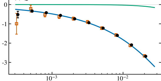
(a) Q^2 = 1.14 \text{ GeV}^2
