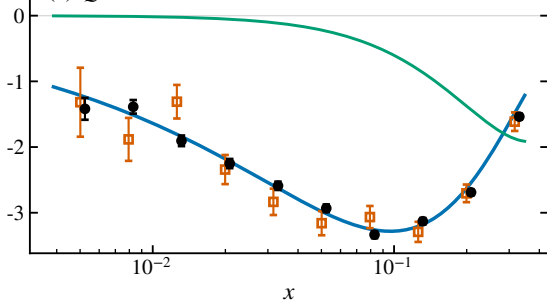
(b) Q^2 = 14.3 \text{ GeV}^2
