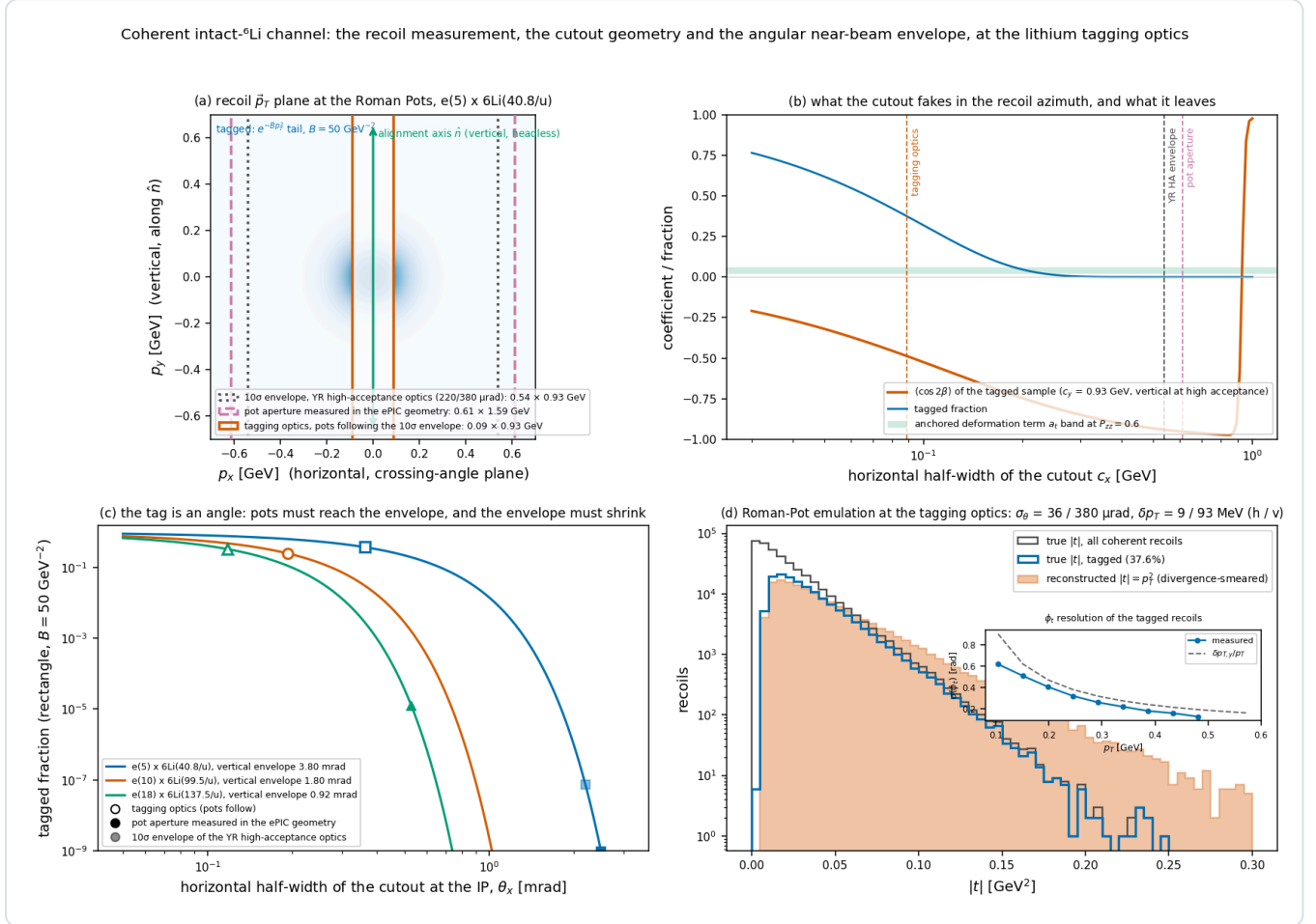
Figure 3 — the coherent measurement quantified ( 5 \times 40.8 , reco_chain_figures.py ). (a) The recoil p_T plane with the exponential coherent spectrum and the three cutouts: the Yellow Report high-acceptance 10\sigma envelope, the pot aperture measured in the ePIC geometry, and the tagging optics with pots following the envelope. (b) (\cos 2\beta) of the tagged sample about the vertical spin axis and the tagged fraction versus the horizontal half-width of the cutout, against the anchored deformation band. (c) Tagged fraction versus the horizontal half-angle at the interaction point for the three configurations, with the three cutouts marked; the markers below 10^{-9} are off the axis, and the aperture marker at 18 \times 137.5 lies inside the envelope that binds there. (d) The Roman-Pot emulation at the tagging optics: true, tagged and reconstructed |t| , and (inset) the \phi_t resolution, dominated by the 93 MeV vertical divergence. The tagged fraction the panel prints, 37.6%, is per recoil above t_{\text{min}} ; Table 5's 36% is the same Monte Carlo and the same cutout counted per recoil produced, the 3.3% between them being the draws the t_{\text{min}} cut removes.
