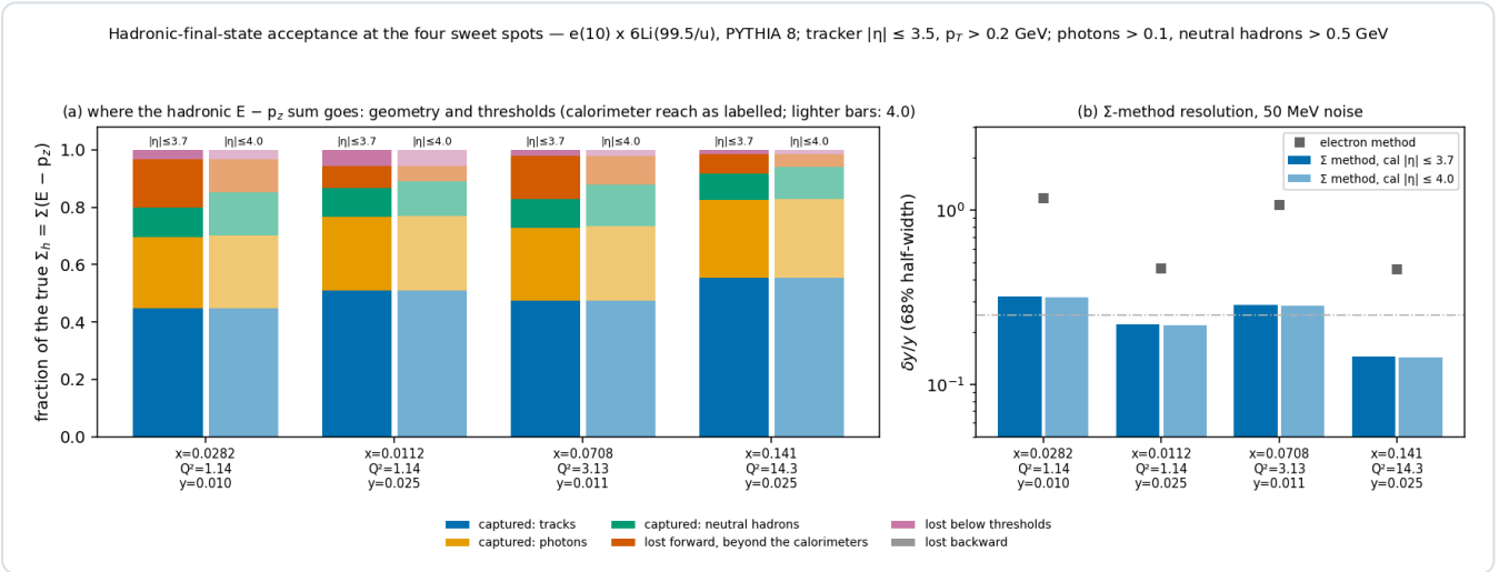
Figure 2 — where the hadronic E - p_z sum goes ( e10 \times {}^6\text{Li}99.5 , PYTHIA 8, hfs_acceptance.py ). (a) The true \Sigma_h by fate — captured as tracks, photons and HCal objects; lost forward beyond the calorimeters, below threshold, or backward — for a calorimeter reach of |\eta| \leq 3.7 (full) and the ePIC nominal 4.0 (light). (b) The \Sigma -method \delta y/y through the full response for both reaches: the extra reach moves the bias, not the resolution.
