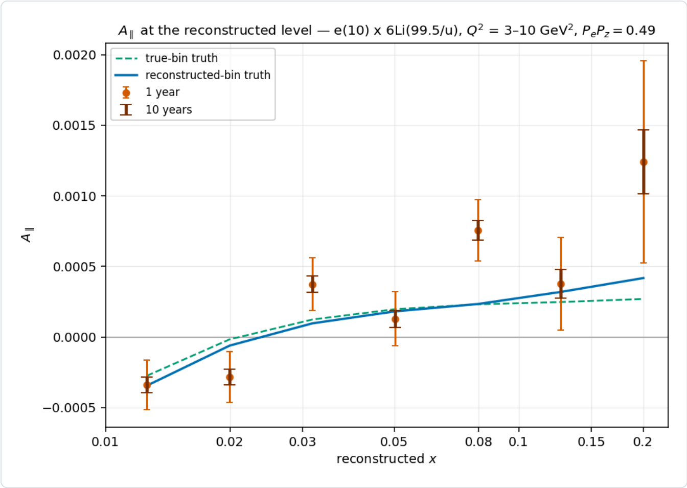
Figure 8 — A_{\parallel} at the reconstructed level (the same response and bins, P_e P_z = 0.49 , electron-helicity flips; money_azz_reco.py --observable apar ). The asymmetry crosses zero between x = 0.02 and 0.03 on this g_1 model, so the migration is quoted in units of the one-year error rather than as a ratio; the one-year errors run 1.8 \times 10^{-4} to 7.2 \times 10^{-4} .
