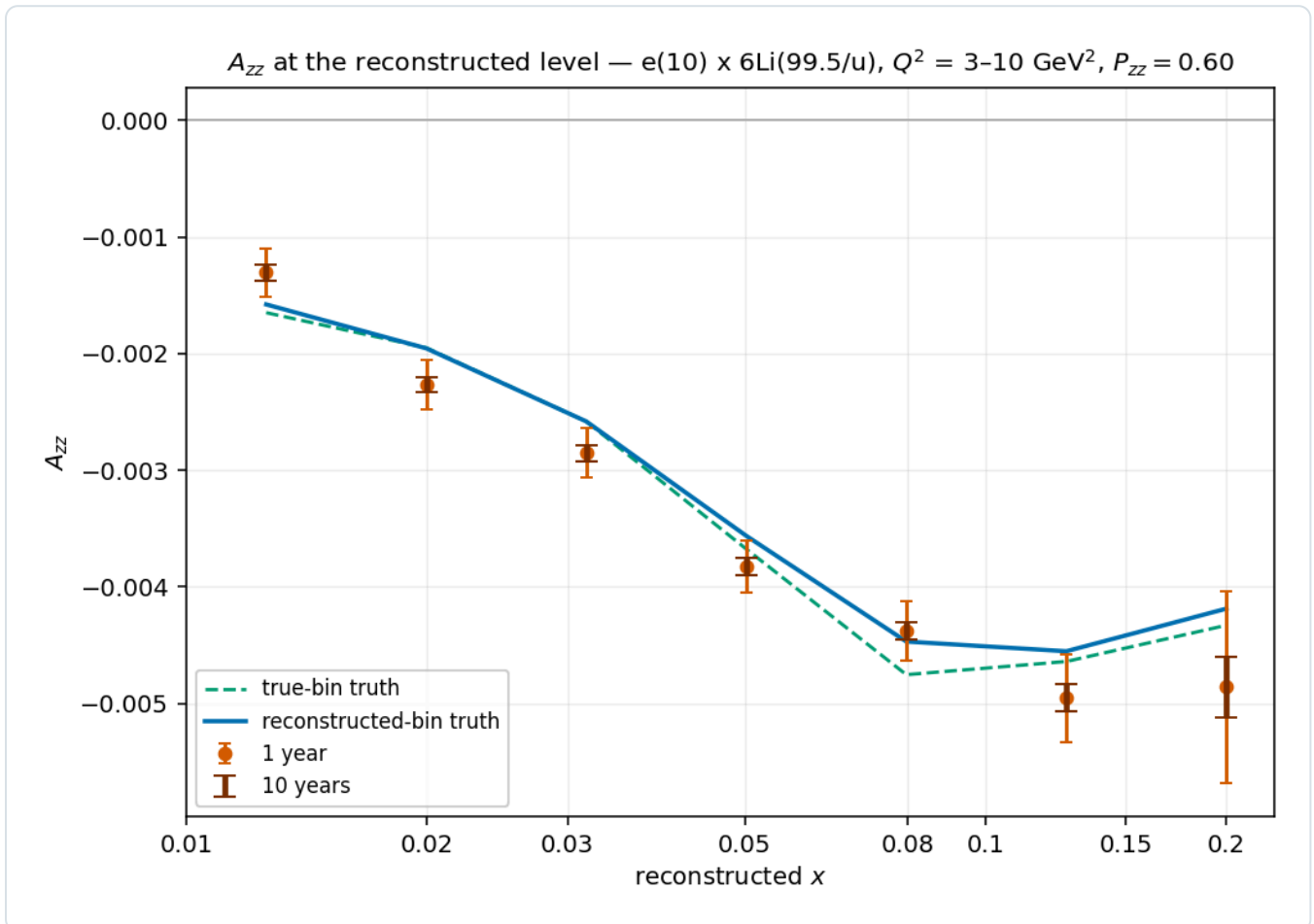
Figure 7 — A_{zz} at the reconstructed level ( e10 \times {}^6\text{Li}99.5 , P_{zz} = 0.6 , tensor-thirds fills, toy b_1 ; money_azz_reco.py ). Seven reconstructed x bins of the Q^2 = 3\text{--}10 \text{ GeV}^2 slice, each holding 8 \times 10^6\text{--}1.4 \times 10^8 events in one year, with one-year (thin) and ten-year (thick) statistical bars, against the reconstructed-bin truth and the true-bin truth. A_{zz} deepens from -1.6 \times 10^{-3} at x = 0.013 to -4.6 \times 10^{-3} at x = 0.13 and turns over to -4.2 \times 10^{-3} at the last bin, x = 0.20 ; the one-year errors are 2.0 \times 10^{-4} at the low- x end and 8.3 \times 10^{-4} at that last bin, where the slice holds 8 \times 10^6 events.
