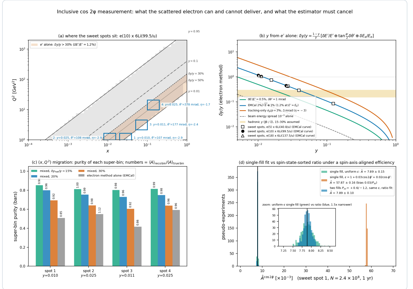
Figure 4 — the inclusive measurement quantified ( e(10) \times 6\text{Li}99.5 , reco_chain_figures.py ). (a) The analysis acceptance with iso- y lines and the four sweet-spot super-bins; the shaded band is where the electron alone gives \delta y/y > 30\% at a 1.2% energy resolution. (b) The electron-method \delta y/y versus y for calorimeter, tracking and beam-energy-spread inputs, with the sweet spots of the three configurations and the 15–30% hadronic band. (c) Purity of each super-bin for three Gaussian hadronic- y resolutions and for the electron method alone; the numbers are the reconstructed-bin over true-bin amplitude; they are migration purities — the electron smearing and the hadronic y alone, without the reconstructed-level analysis window or \epsilon_{\text{elD}} — and are not on the footing of the purities of Table 4, which are through the full selection. (d) Four hundred pseudo-experiments of the spot-1 super-bin at one year, generated at its truth-level count N = 2.4 \times 10^8 (Table 4's 1.6 \times 10^8 is the reconstructed one, so the errors here are 0.10 rather than 0.12 \times 10^{-3} ): the single-fill fit under a uniform efficiency (green), the same under \epsilon = 1 + 0.03 \cos 2\phi' + 0.02 \cos \phi' (vermillion, biased by 0.03/P_{zz} ), and the two-state ratio under that efficiency (blue, unbiased and 1.5 \times narrower).
