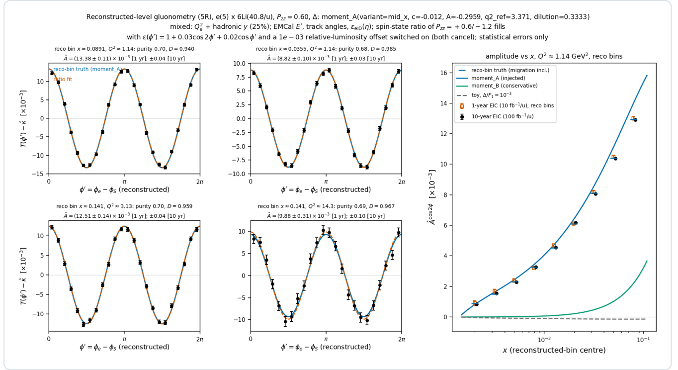
Figure 5 — the low configuration reaches x \approx 0.1 at low Q^2 (e5 \times ^6\text{Li}40.8/u , P_{zz} = 0.6 , model A, mixed method with the 25% Gaussian hadronic-y stand-in, otherwise the settings of money plot 5R; money_cos2phi_reco.py --config 0 ). Left: the acceptance-free modulation T(\phi') - \hat{k} per unit P_{zz} in the four sweet-spot super-bins, of which the first sits at x = 0.089 and the last two at x = 0.141 , with the reconstructed-bin truth and the fit. Right: the amplitude in reconstructed x bins along the Q^2 = 1.14 GeV 2 slice.
