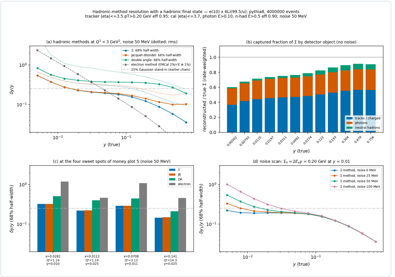
Figure 1 — hadronic-method resolution ( e10 \times {}^6\text{Li}99.5 , PYTHIA 8, hfs_resolution.py ). (a) \delta y/y (68% half-width; dotted: rms) of the \Sigma , Jacquet-Blondel and double-angle methods at Q^2 < 3 \text{ GeV}^2 with 50 MeV of noise, against the electron method and the 25% stand-in of the earlier chain. (b) Captured fraction of \Sigma by detector object, rate-weighted, no noise. (c) The four sweet spots. (d) The \Sigma -method resolution for 0, 25, 50 and 100 MeV of noise: the floor decides the y \approx 0.01 bins.
