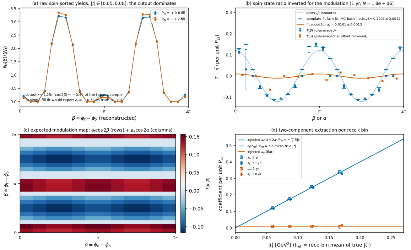
Money plot 6R — the coherent channel at the reconstructed level. (a) Raw spin-sorted yields versus the reconstructed recoil azimuth \beta for the lowest |t| bin: the cutout shape dominates both fills identically. (b) The modulation T(\beta) and T(\alpha) recovered from the spin-state ratio ( T(\alpha) with the a_t offset removed), the template-fit prediction per \beta bin (ticks) and the smooth a_t \cos 2\beta and a_e \cos 2\alpha curves. (c) The expected (noise-free) modulation map in (\alpha, \beta) : rows from the deformation term, columns from the gluon-transversity term. (d) Extracted a_t(t_{\text{ref}}) and a_e per reco |t| bin (1 yr open, 10 yr filled) against the injected curves.
