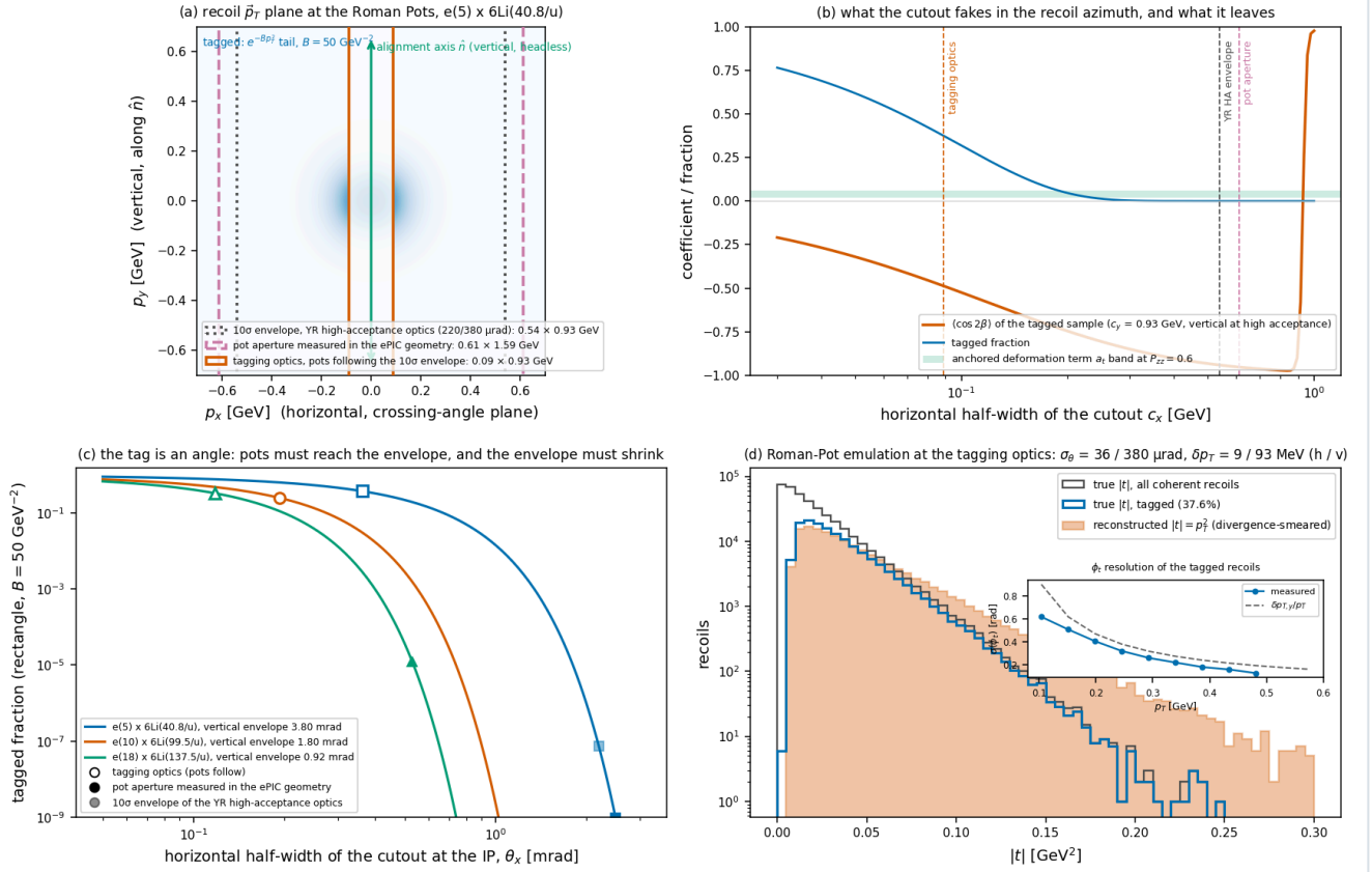
Figure 3 — the coherent measurement quantified ( 5 \times 40.8 , reco_chain_figures.py ). (a) The recoil p_T plane with the exponential coherent spectrum and the three cutouts: the Yellow Report high-acceptance 10\sigma envelope, the pot aperture measured in the ePIC geometry, and the tagging optics with pots following the envelope. (b) \langle \cos 2\beta \rangle of the tagged sample about the vertical spin axis and the tagged fraction versus the horizontal half-width of the cutout, against the anchored deformation band. (c) Tagged fraction versus the horizontal half-angle at the interaction point for the three configurations, with the three cutouts marked. (d) The Roman-Pot emulation at the tagging optics: true, tagged and reconstructed |t| , and (inset) the \phi_t resolution, dominated by the 93 MeV vertical divergence.
