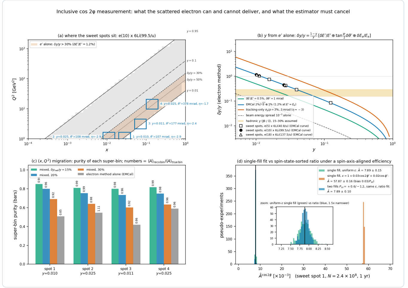
Figure 4 — the inclusive measurement quantified ( e10 \times 6\text{Li}99.5 , reco_chain_figures.py ). (a) The analysis acceptance with iso- y lines and the four sweet-spot super-bins; the shaded band is where the electron alone gives \delta y/y > 30\% at a 1.2% energy resolution. (b) The electron-method \delta y/y versus y for calorimeter, tracking and beam-energy-spread inputs, with the sweet spots of the three configurations and the 15–30% hadronic band. (c) Purity of each super-bin for three Gaussian hadronic- y resolutions and for the electron method alone; the numbers are the reconstructed-bin over true-bin amplitude. (d) Four hundred pseudo-experiments of the spot-1 super-bin at one year: the single-fill fit under a uniform efficiency (green), the same under \epsilon = 1 + 0.03 \cos 2\phi' + 0.02 \cos \phi' (vermillion, biased by 0.03/P_{zz} ), and the two-state ratio under that efficiency (blue, unbiased and 1.5\times narrower).
