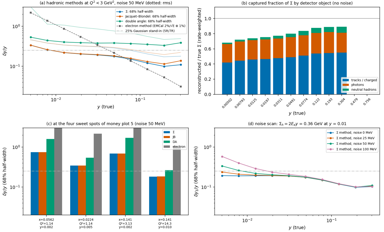
Figure 3 — hadronic-method resolution with a hadronic final state (e10 × 6 Li50, PYTHIA 8 , 4 M e + p and e + n events, hfs_resolution.py ). (a) \delta y/y (68% half-width; dotted: rms) of the \Sigma , Jacquet-Blondel and double-angle methods at Q^2 < 3 \text{ GeV}^2 with the default response and 50 MeV noise, against the electron method and the 25% stand-in. (b) Captured fraction of \Sigma by detector object, no noise. (c) The four sweet spots. (d) The \Sigma -method resolution for 0, 25, 50 and 100 MeV of calorimeter noise.
