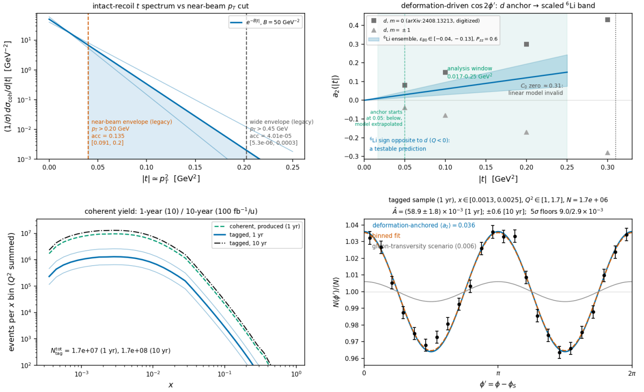
Figure 5 — the coherent channel e^6\text{Li} \rightarrow e'X^6\text{Li}(\text{g.s.}) at e(10 \text{ GeV}) \times ^6\text{Li}(99.5 \text{ GeV}/\text{u}) , P_{zz} = 0.60 , for a 0.20 GeV near-beam envelope. (a) Recoil t spectrum with the slope band and the 0.20 and 0.45 GeV cuts ( 13.5\% and 4 \times 10^{-5} ); the panel's optics labels are the proton optics the two cuts were first derived from, neither of which is an available ^6\text{Li} optics ( \$6.1 ). (b) Digitized deuteron a_2 per m state [10] against the scaled ^6\text{Li} ensemble band (sign flip predicted), with the analysis window 0.017–0.25 GeV ^2 — the reconstructed binning of money plot 6R (Report 2 §5.2), whose lower edge is a choice of the analysis above the tagging-optics aperture floor of 0.0064–0.0098 GeV ^2 and not the floor itself — the marker at |t| = 0.05 \text{ GeV}^2 where the digitized anchor begins, below which the band, and the a_t truth of the four reconstructed bins whose t_{\text{ref}} falls there, are the linear model extrapolated, and the form-factor-zero exclusion. (c) Tagged yield versus x for both programmes with the f_0 band. (d) \phi' pseudo-data (one-year statistics) at \langle a_2 \rangle = 0.036 with the flat gluon-transversity scenario (grey); extraction \hat{A} \pm 1.8 \times 10^{-3} (one year), \pm 0.6 \times 10^{-3} (ten years) per unit P_{zz} .
