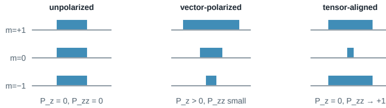
Figure 1 — populations of the three spin projections for an unpolarized, a vector-polarized and a tensor-aligned spin-1 fill. The tensor moment measures the m = \pm 1 population against m = 0 and is independent of the vector one.
