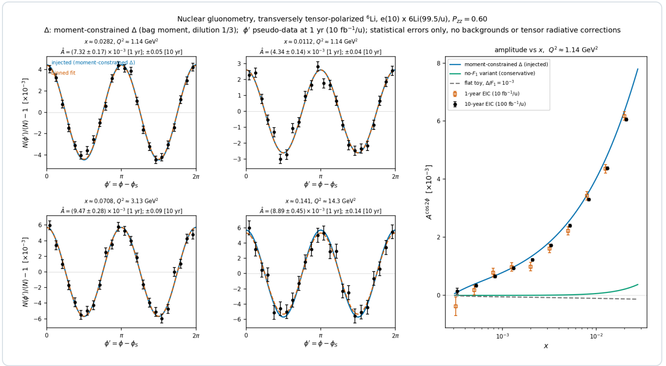
Figure 3 — projected extraction of \Delta \cdot \cos 2\phi' pseudo-data (one EIC year, P_{zz} = 0.6 ) in the four highest-significance ( x , Q^2 ) bins, with the injected moment-constrained \Delta model and the binned fit; right, the extracted amplitude versus x against alternative model readings. The precision distinguishes between the models rather than only from zero. The reconstructed-level version uses the spin-state ratio in reconstructed bins [5].
