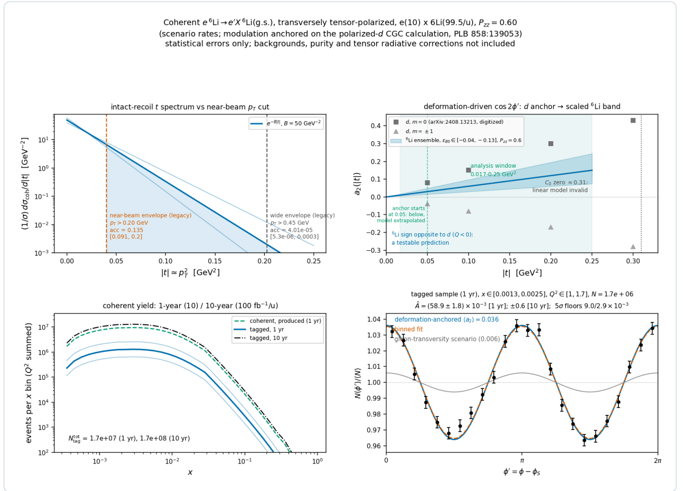
Figure 5 — the coherent channel e {}^6\text{Li} \rightarrow e' X {}^6\text{Li}(\text{g.s.}) at e(10 \text{ GeV}) \times {}^6\text{Li}(99.5 \text{ GeV}/u) , P_{zz} = 0.60 , for a 0.20 GeV near-beam envelope; the four panels are titled rather than lettered and run (a) top left, (b) top right, (c) bottom left, (d) bottom right. (a) Recoil t spectrum with the slope band and the 0.20 and 0.45 GeV cuts ( 13.5\% and 4 \times 10^{-5} ); both envelopes, which the panel marks legacy , are the proton optics the two cuts were first derived from — the 0.20 and 0.45 GeV cuts of a 275 GeV proton — neither of which is an available {}^6\text{Li} optics ( \$6.1 ). (b) Digitized deuteron a_2 per m state [10] against the scaled {}^6\text{Li} ensemble band (sign flip predicted), with the analysis window 0.017\text{--}0.25 \text{ GeV}^2 — the reconstructed binning of money plot 6R (Report 2 §5.2), whose lower edge is a choice of the analysis above the tagging-optics aperture floor of 0.0079\text{--}0.0132 \text{ GeV}^2 and not the floor itself — the marker at |t| = 0.05 \text{ GeV}^2 where the digitized anchor begins, below which the band, and the a_t truth of the four reconstructed bins whose t_{\text{ref}} falls there, are the linear model extrapolated, and the form-factor-zero exclusion. (c) Tagged yield versus x for both programmes with the f_0 band. (d) \phi' pseudo-data (one-year statistics) at \langle a_2 \rangle = 0.036 with the flat gluon-transversity scenario (grey); extraction \hat{A} \pm 1.8 \times 10^{-3} (one year), \pm 0.6 \times 10^{-3} (ten years) per unit P_{zz} .
