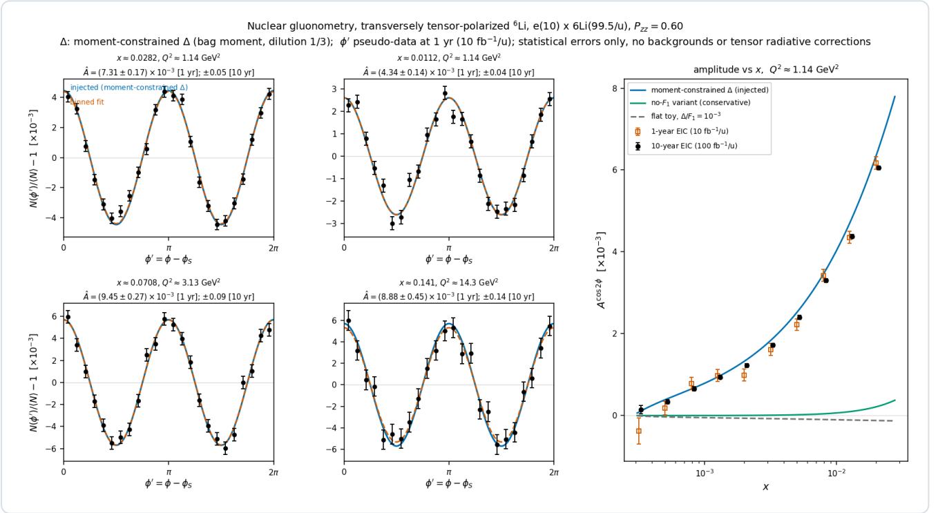
Figure 3 — projected extraction of \Delta . \cos 2\phi pseudo-data (one EIC year, P_{zz} = 0.6 ) in the four highest-significance (x, Q^2) bins, with the injected moment-constrained \Delta model and the binned fit; right, the extracted amplitude versus x at Q^2 \approx 1.14 \text{ GeV}^2 , one-year (open) and ten-year (filled), against alternative model readings. The panels' abscissa \phi' is the \phi of §4.2, written on the axis as the lab azimuth of the scattered electron minus that of the spin axis. The precision distinguishes between the models rather than only from zero. The reconstructed-level version uses the spin-state ratio in reconstructed bins [5].
