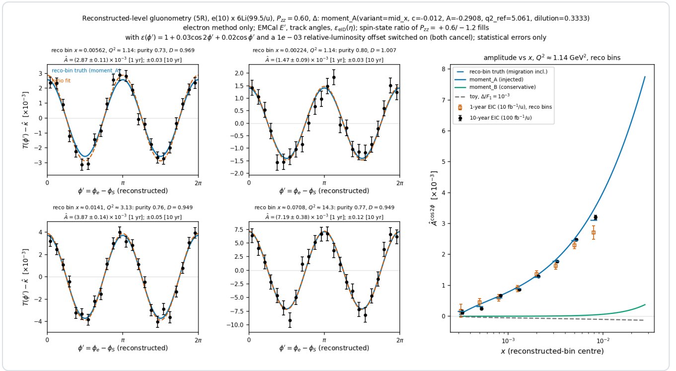
Figure 6 — the electron method alone above y = 0.05 ( e(10) \times \text{Li}(99.5, P_{ZZ} = 0.6, \text{model A}, Q^2_e and y_e from the scattered electron with no hadronic sum, reconstructed y \geq 0.05 , otherwise the settings of money plot 5R; money_cos2phi_reco.py --y-method electron --y-min 0.05 ). Left: the acceptance-free modulation T(\phi') - \hat{k} per unit P_{ZZ} in the four sweet-spot super-bins of that window, with the reconstructed-bin truth and the fit. Right: the amplitude in reconstructed x bins along the Q^2 = 1.14 \text{ GeV}^2 slice.
