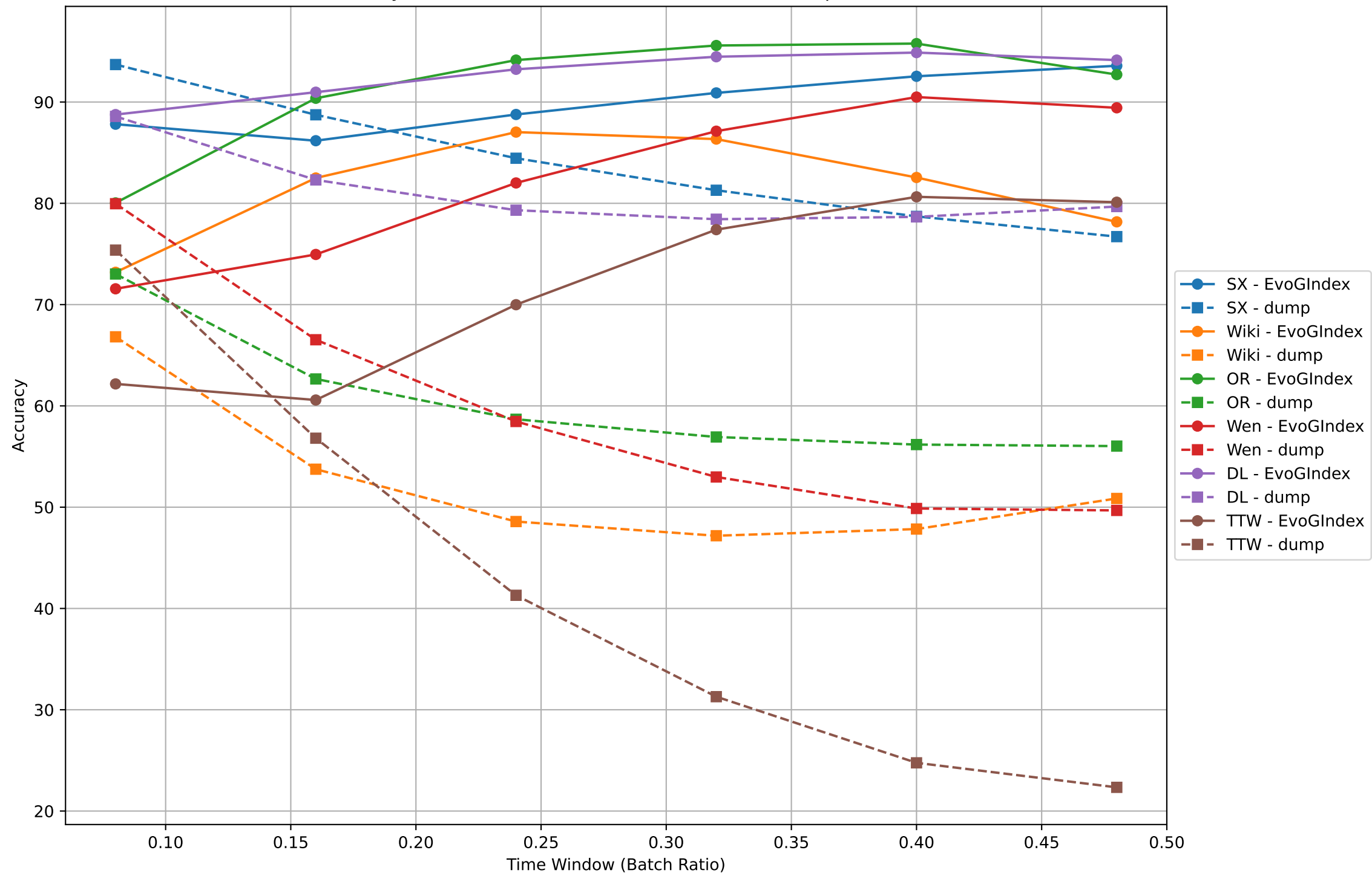
Accuracy vs Time Window (Each Dataset Uses a Unique Color)
