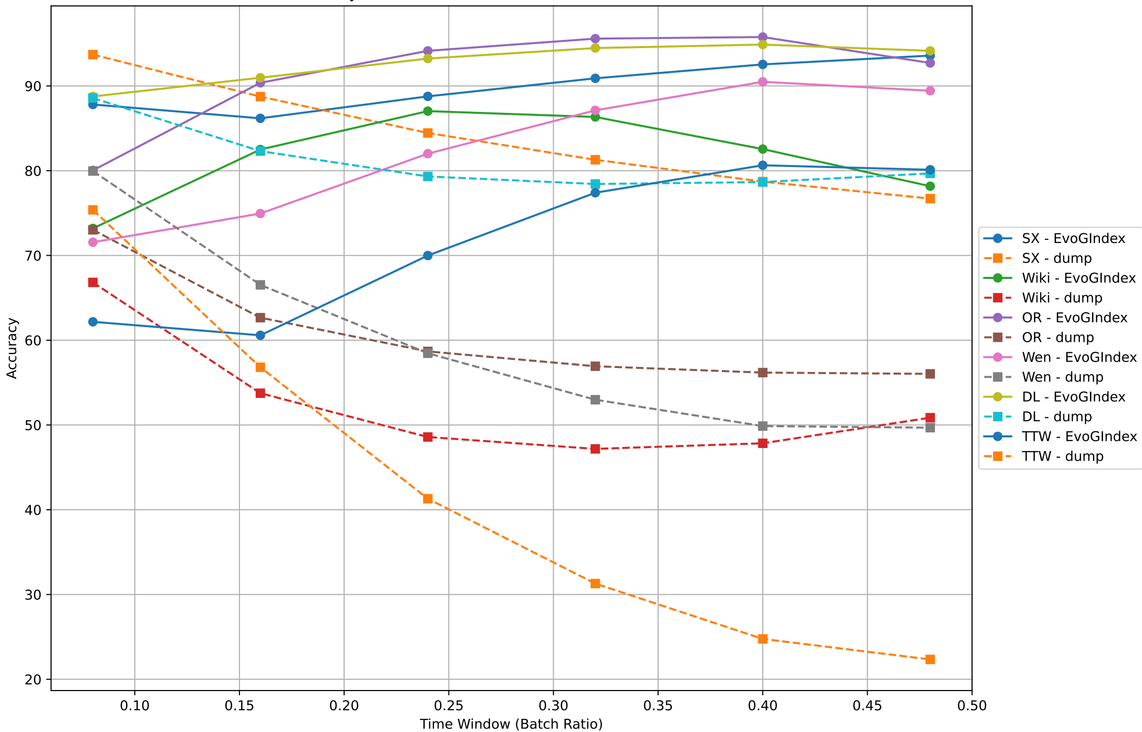
Accuracy vs Time Window (All Benchmarks on One Plot)
