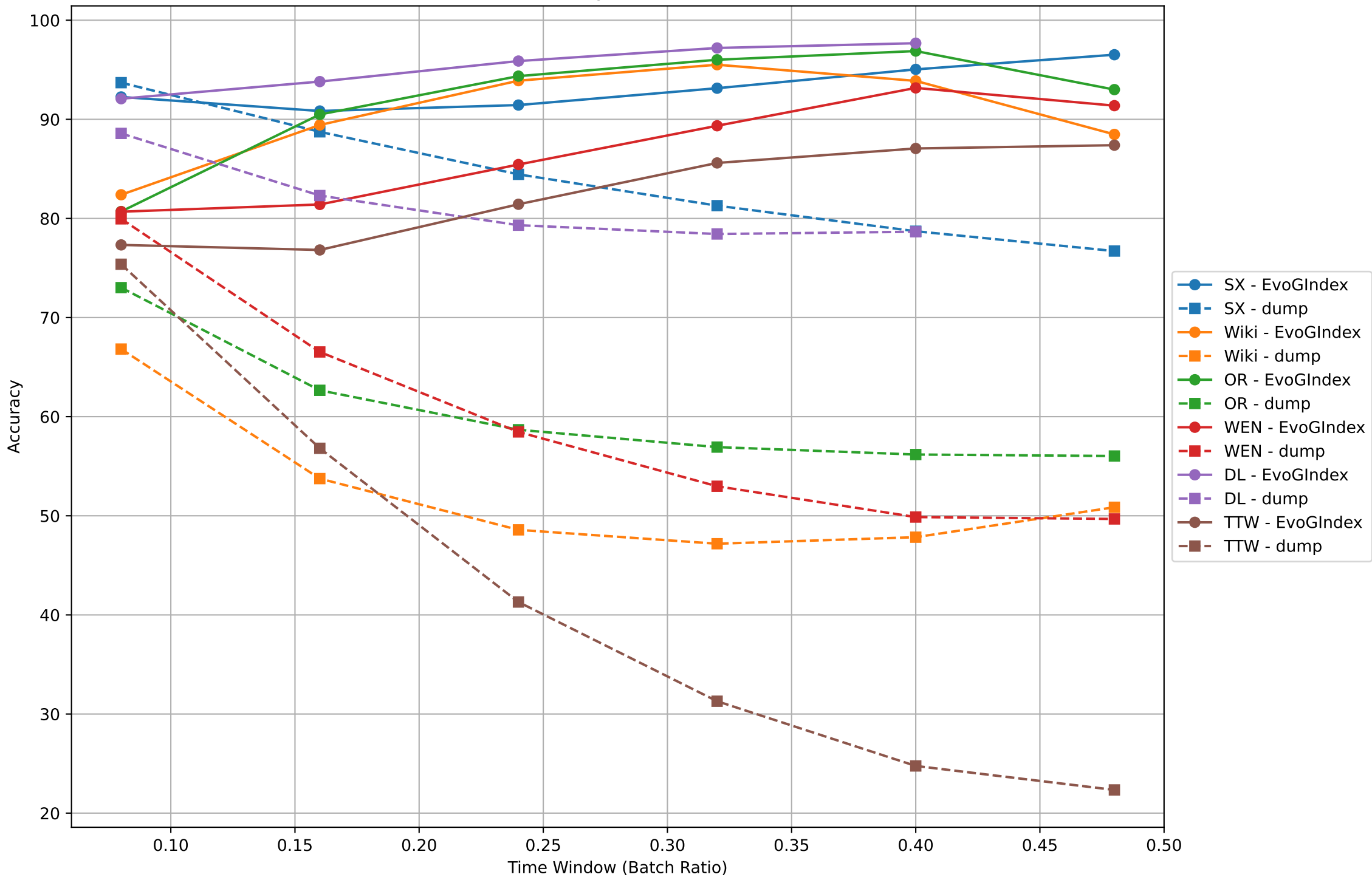
SSSP Accuracy vs Time Window
