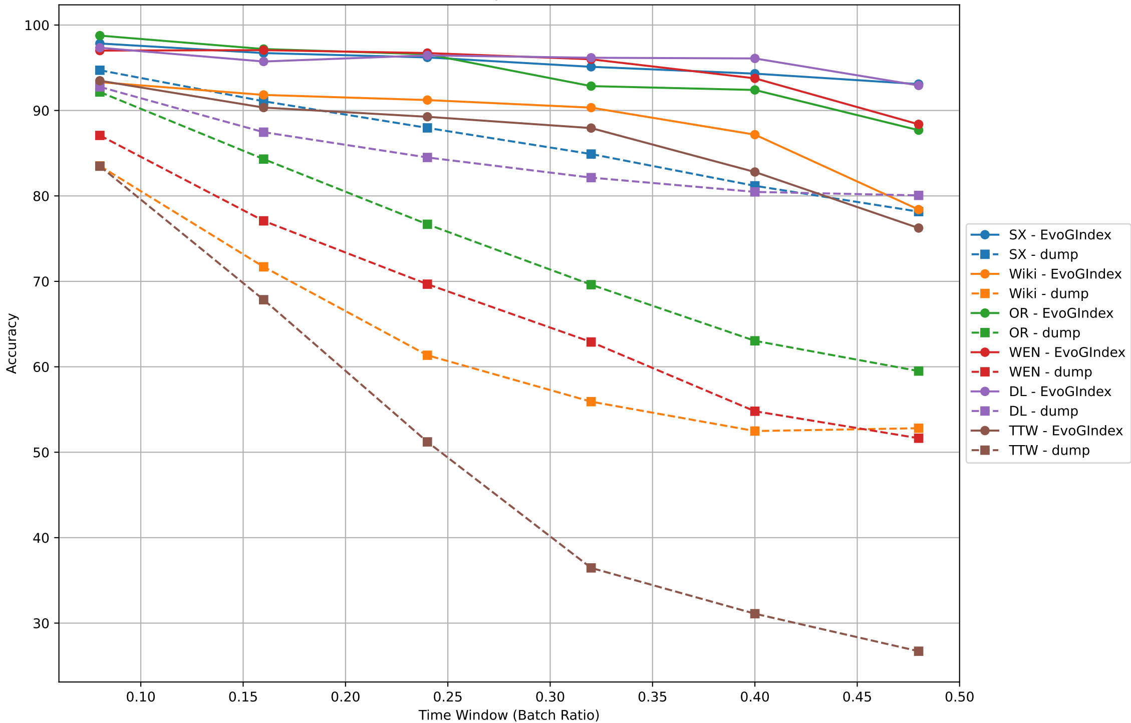
SSWP Accuracy vs Time Window
