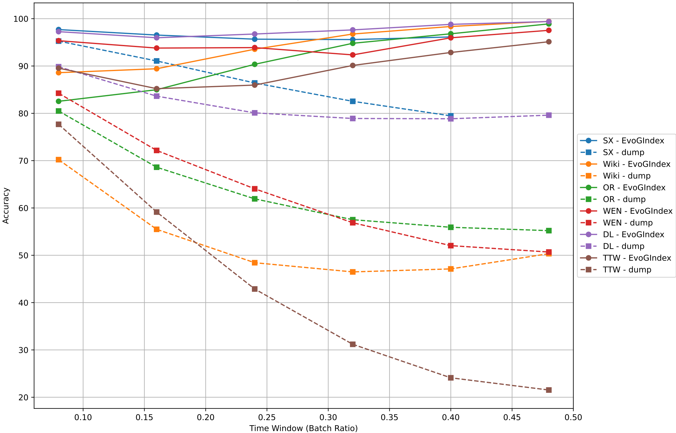
Viterbi Accuracy vs Time Window
