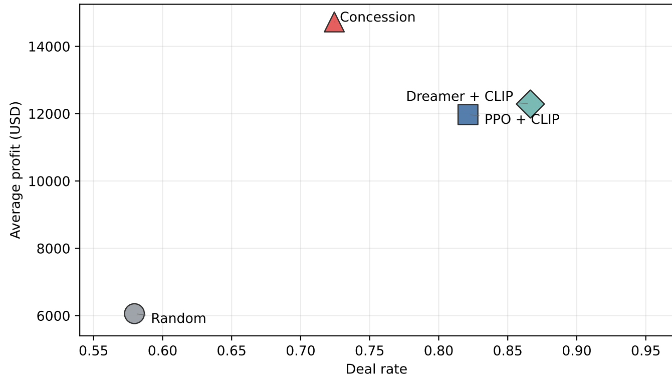
Agreement-profit trade-off in the benchmark
