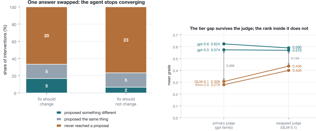
Figure 2: Left: swapping one authored answer does not redirect the agent, it stops it—and the collapse is worse in the column where the diagnosis was not supposed to move. Right: all four rows under two judges, same transcripts, same written rubrics. They disagree substantially about absolute quality; the tier separation survives both and the ordering within a tier does not.
