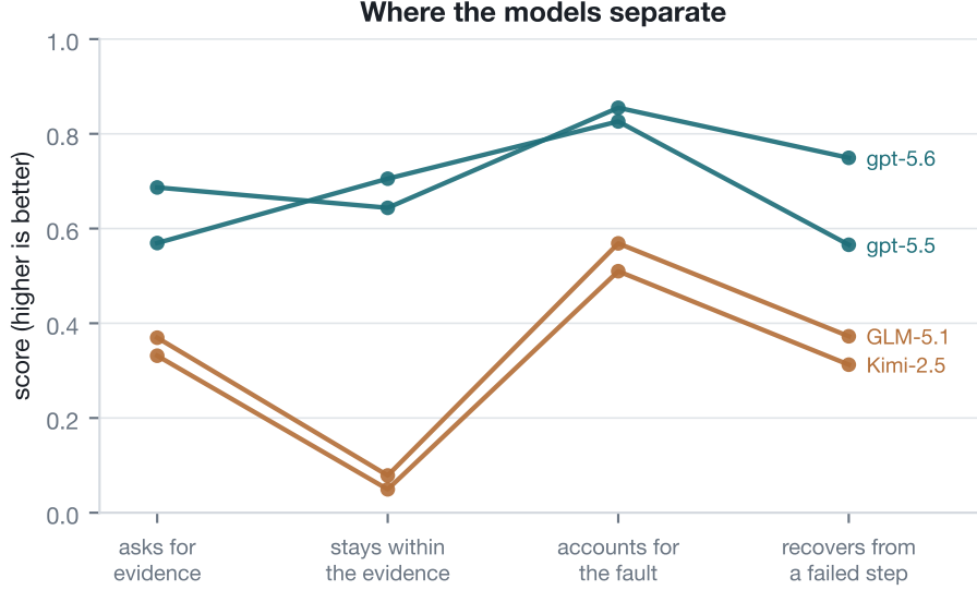
Figure 2: The tiers separate on all four rubrics and never cross. The deepest gap is staying inside the evidence.
