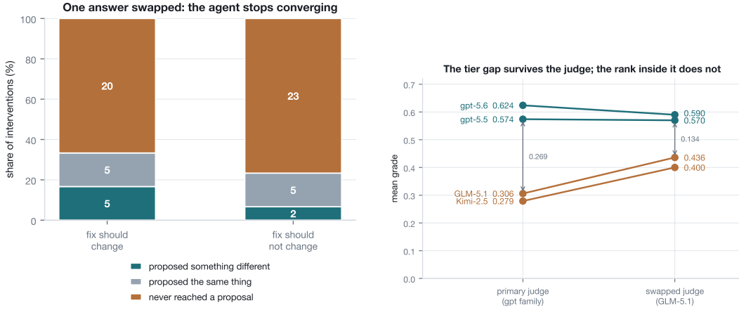
Figure 3: Left: swapping one authored answer does not redirect the agent, it stops it—and the collapse is worse in the column where the diagnosis was not supposed to move. Right: all four rows under two judges, same transcripts, same written rubrics. They disagree substantially about absolute quality; the tier separation survives both and the ordering within a tier does not.
