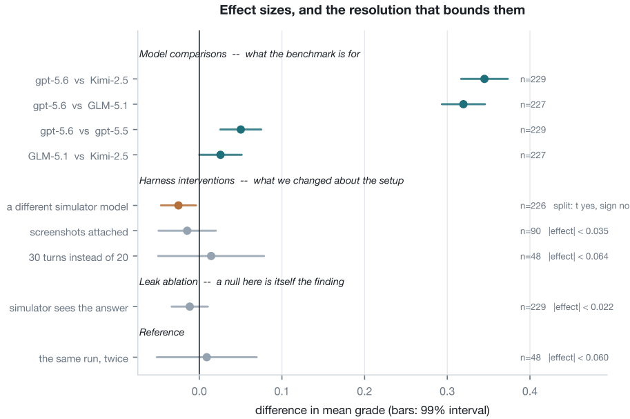
Figure 4: Every comparison, with a 99% interval, grouped by what a null would mean. Both rows we re-ran at full corpus moved: the simulator swap from -0.001 to -0.025 (orange—the paired t clears our threshold while the sign test does not, so it is not called), and the leak ablation to -0.011 , bounding at 0.022 the grade effect of handing the simulator the answer, which is why the score cannot detect leakage. Rows are coloured by the paper’s ruling rule rather than by whether the interval clears zero. Each uncalled row is annotated with the effect it can exclude; the remaining n = 48 rows exclude only \pm 0.06 .
