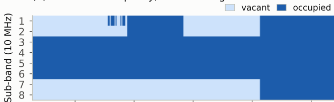
(c) Prediction error (decision accuracy 0.94)
