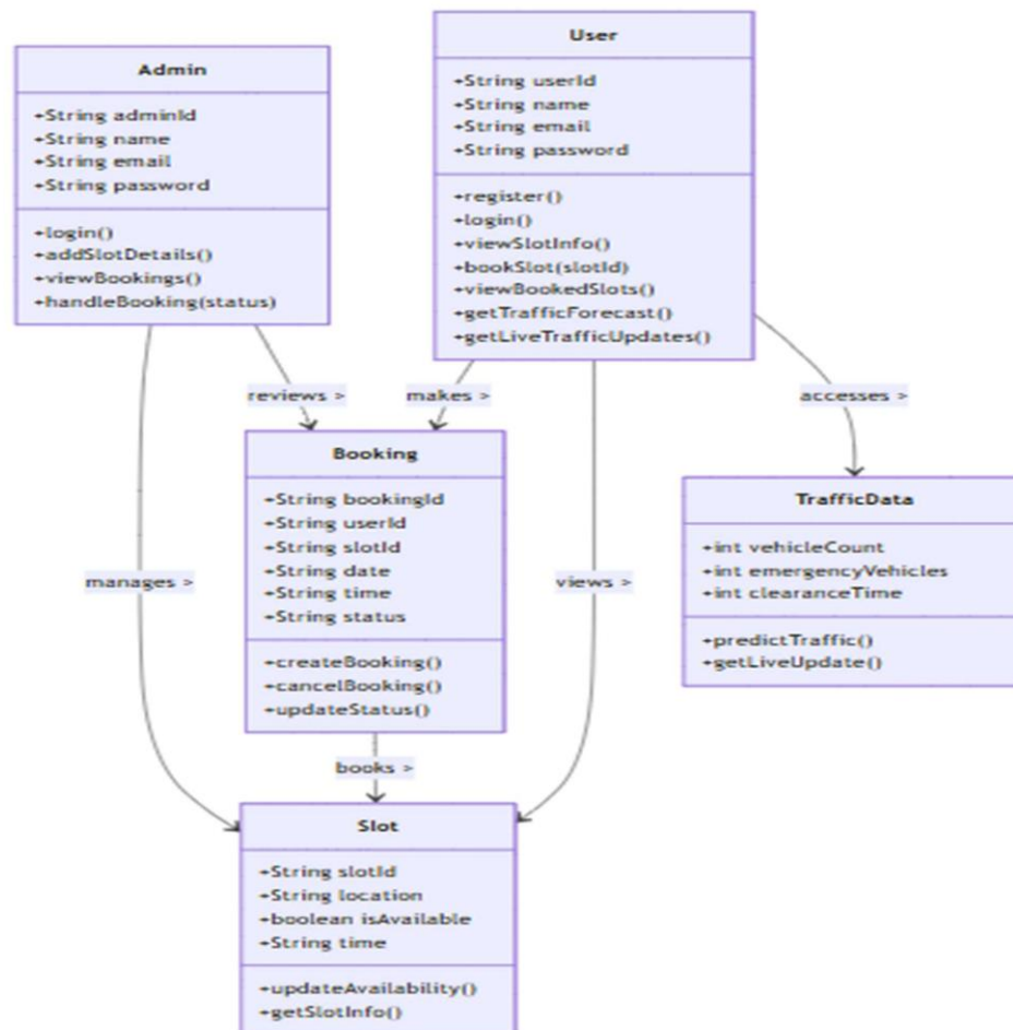
Figure 6.2: Class Diagram
