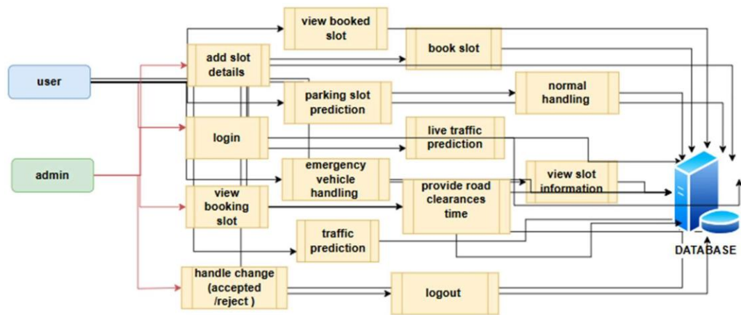
Figure 6.9: DFD Diagram
